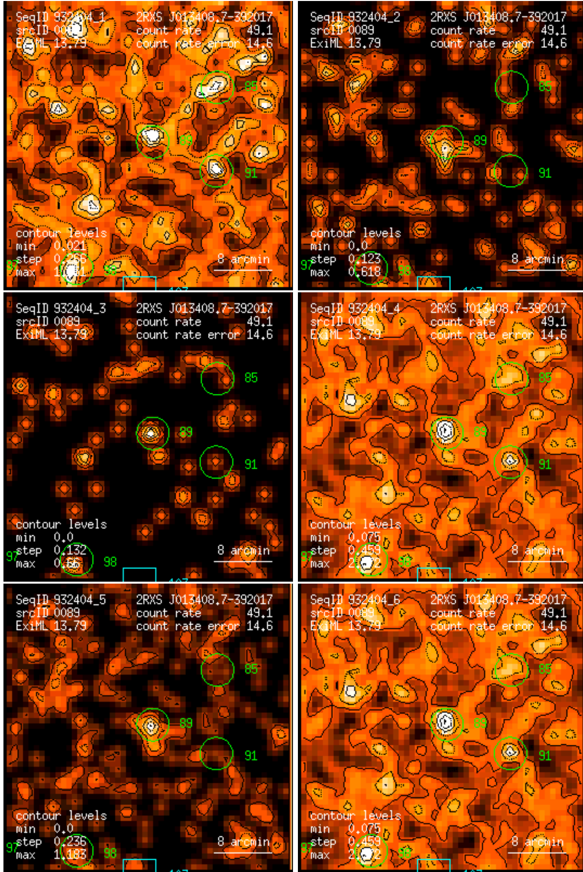
Figure 89: RASS 932404: detection 0089: band rate images, Gaussian filter: (1) PSPC channels 11 – 41, (2) 52 – 90, (3) 91 – 201, (4) 11 – 235, (5) 52 – 201, (6) 11 – 201. Broad band rates in counts/ks. Band rate contour levels in counts/ks/arcmin 2 .
