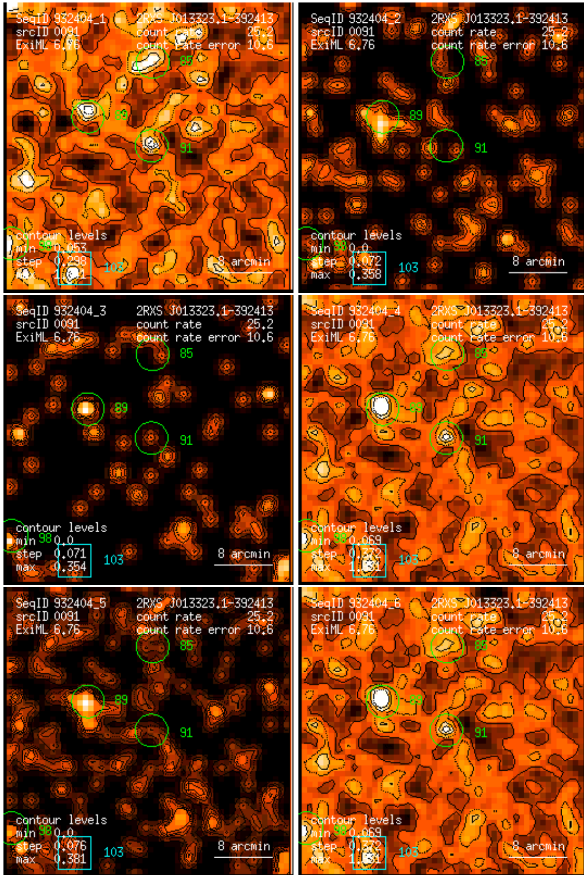
Figure 91: RASS 932404: detection 0091: band rate images, Gaussian filter: (1) PSPC channels 11 – 41, (2) 52 – 90, (3) 91 – 201, (4) 11 – 235, (5) 52 – 201, (6) 11 – 201. Broad band rates in counts/ks. Band rate contour levels in counts/ks/arcmin 2 .
