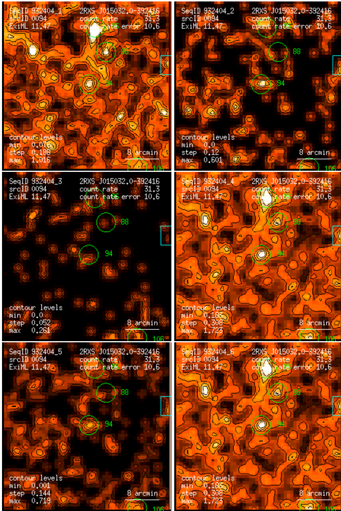
Figure 94: RASS 932404: detection 0094: band rate images, Gaussian filter: (1) PSPC channels 11 – 41, (2) 52 – 90, (3) 91 – 201, (4) 11 – 235, (5) 52 – 201, (6) 11 – 201. Broad band rates in counts/ks. Band rate contour levels in counts/ks/arcmin 2 .
