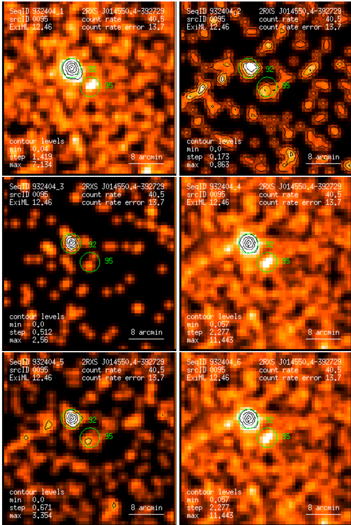
Figure 95: RASS 932404: detection 0095: band rate images, Gaussian filter: (1) PSPC channels 11 – 41, (2) 52 – 90, (3) 91 – 201, (4) 11 – 235, (5) 52 – 201, (6) 11 – 201. Broad band rates in counts/ks. Band rate contour levels in counts/ks/arcmin 2 .
