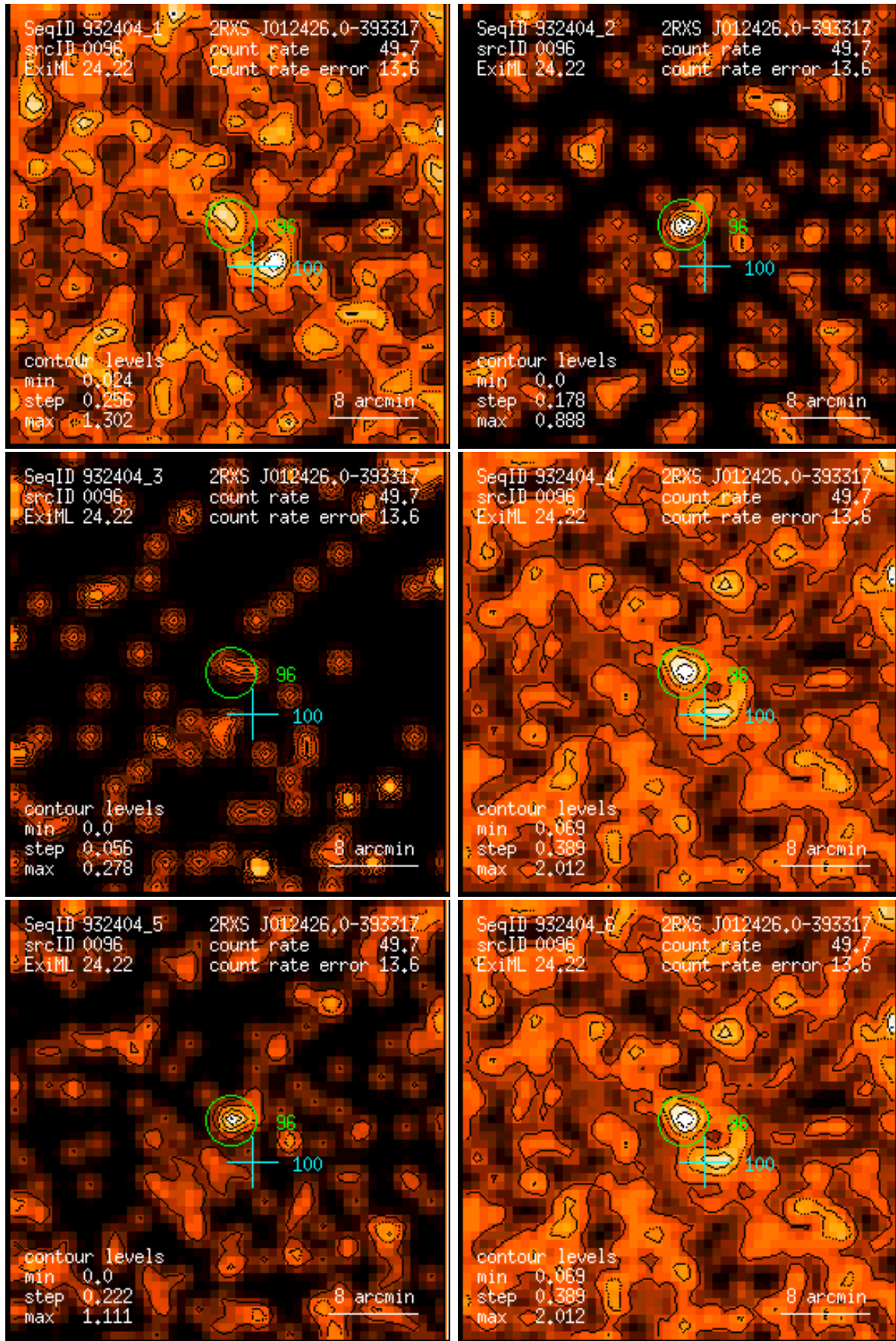
Figure 96: RASS 932404: detection 0096: band rate images, Gaussian filter: (1) PSPC channels 11 – 41, (2) 52 – 90, (3) 91 – 201, (4) 11 – 235, (5) 52 – 201, (6) 11 – 201. Broad band rates in counts/ks. Band rate contour levels in counts/ks/arcmin 2 .
