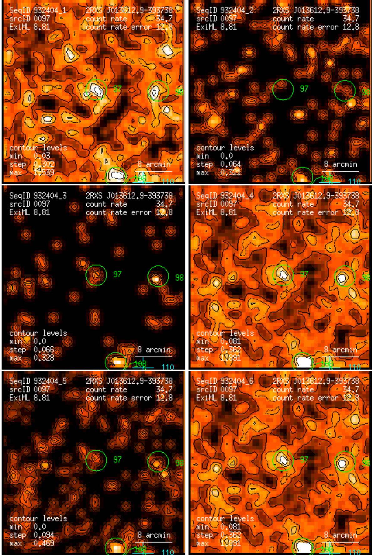
Figure 97: RASS 932404: detection 0097: band rate images, Gaussian filter: (1) PSPC channels 11 – 41, (2) 52 – 90, (3) 91 – 201, (4) 11 – 235, (5) 52 – 201, (6) 11 – 201. Broad band rates in counts/ks. Band rate contour levels in counts/ks/arcmin 2 .
