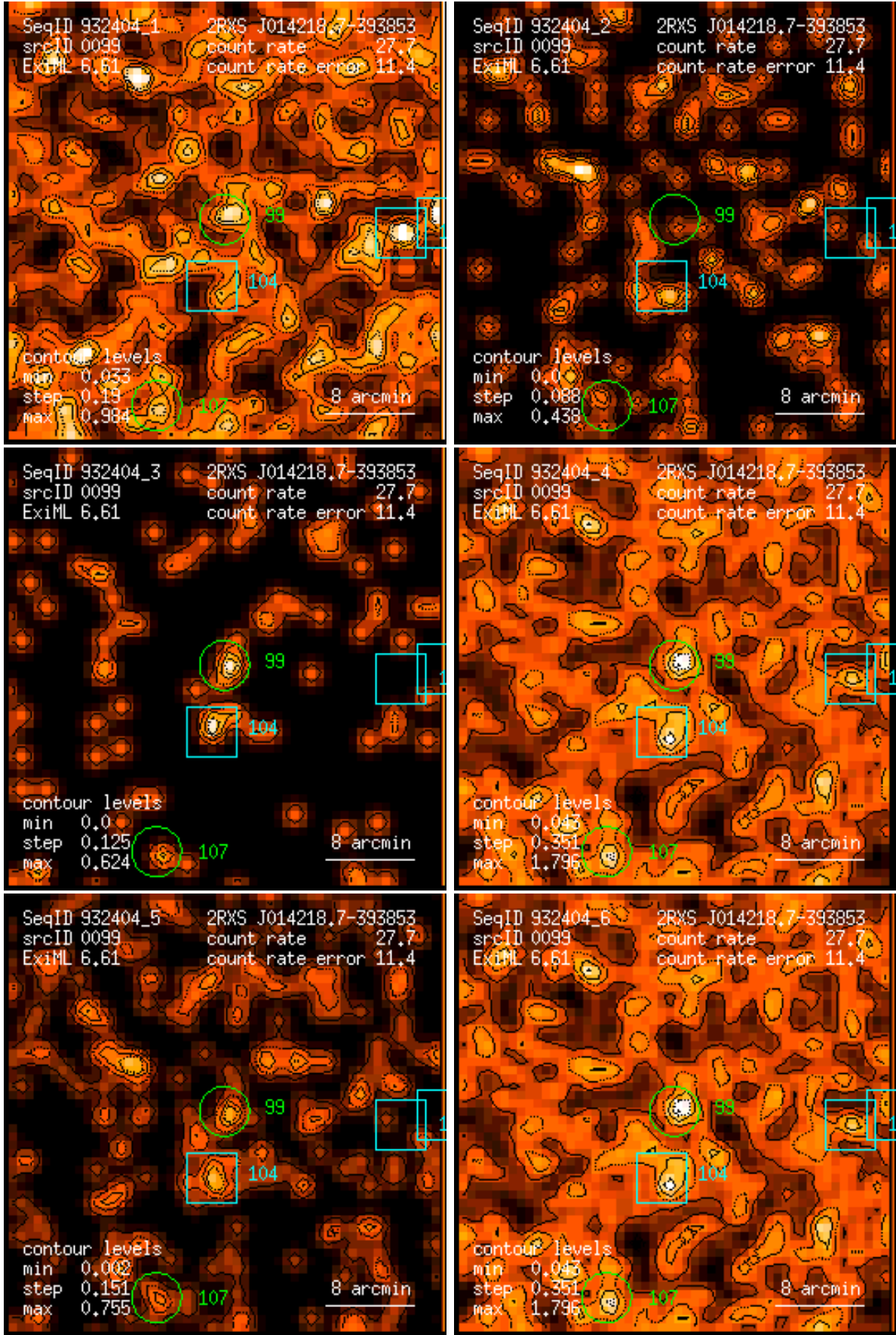
Figure 99: RASS 932404: detection 0099: band rate images, Gaussian filter: (1) PSPC channels 11 – 41, (2) 52 – 90, (3) 91 – 201, (4) 11 – 235, (5) 52 – 201, (6) 11 – 201. Broad band rates in counts/ks. Band rate contour levels in counts/ks/arcmin 2 .
