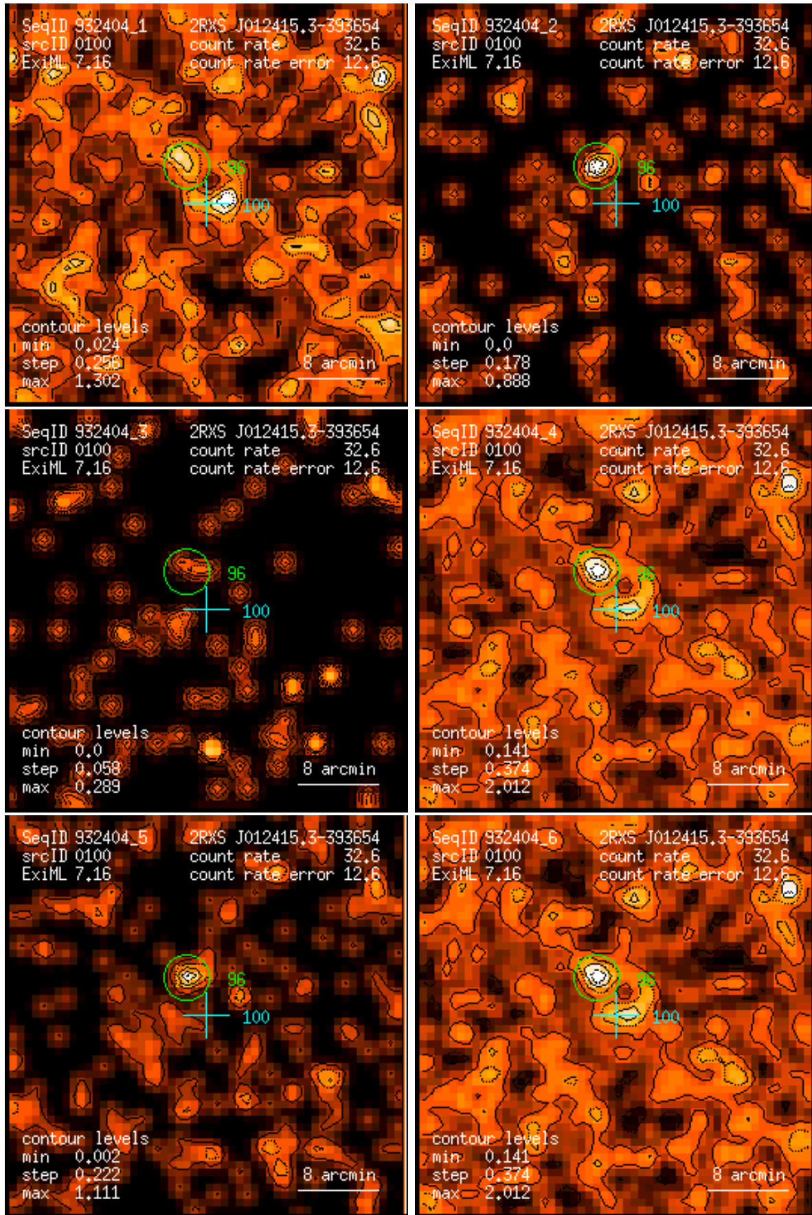
Figure 100: RASS 932404: detection 0100: band rate images, Gaussian filter: (1) PSPC channels 11 – 41, (2) 52 – 90, (3) 91 – 201, (4) 11 – 235, (5) 52 – 201, (6) 11 – 201. Broad band rates in counts/ks. Band rate contour levels in counts/ks/arcmin 2 .
