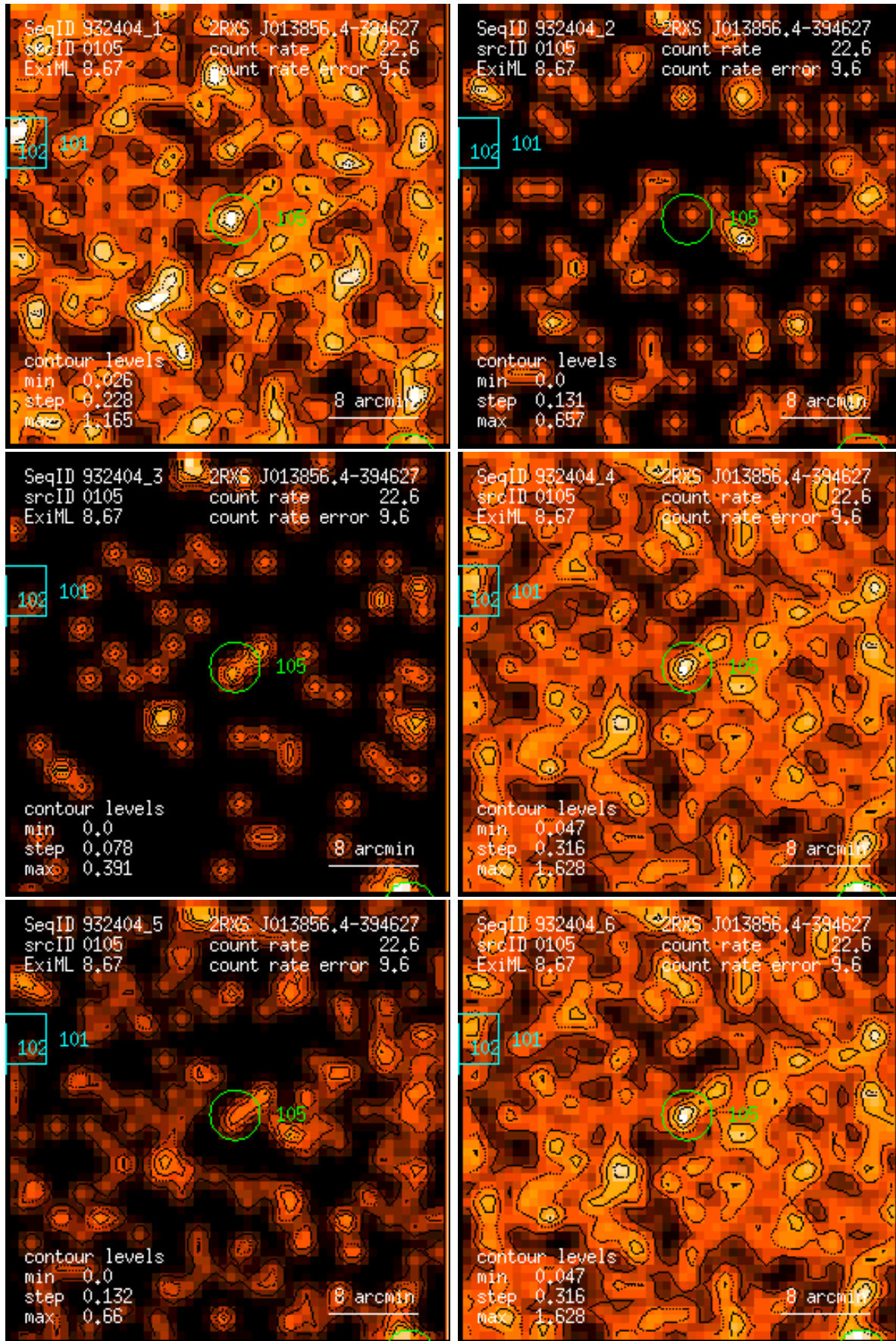
Figure 105: RASS 932404: detection 0105: band rate images, Gaussian filter: (1) PSPC channels 11 – 41, (2) 52 – 90, (3) 91 – 201, (4) 11 – 235, (5) 52 – 201, (6) 11 – 201. Broad band rates in counts/ks. Band rate contour levels in counts/ks/arcmin 2 .
