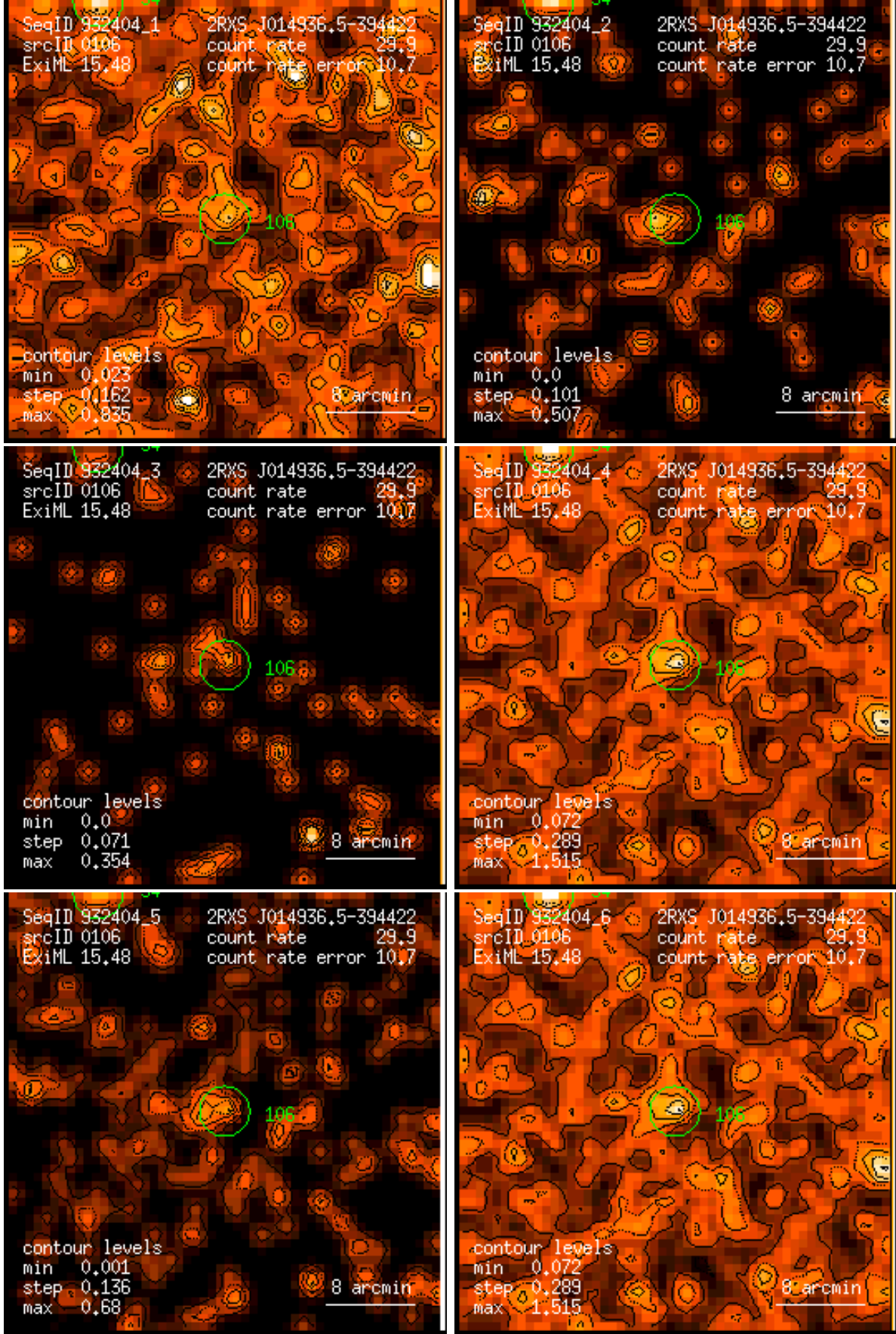
Figure 106: RASS 932404: detection 0106: band rate images, Gaussian filter: (1) PSPC channels 11 – 41, (2) 52 – 90, (3) 91 – 201, (4) 11 – 235, (5) 52 – 201, (6) 11 – 201. Broad band rates in counts/ks. Band rate contour levels in counts/ks/arcmin 2 .
