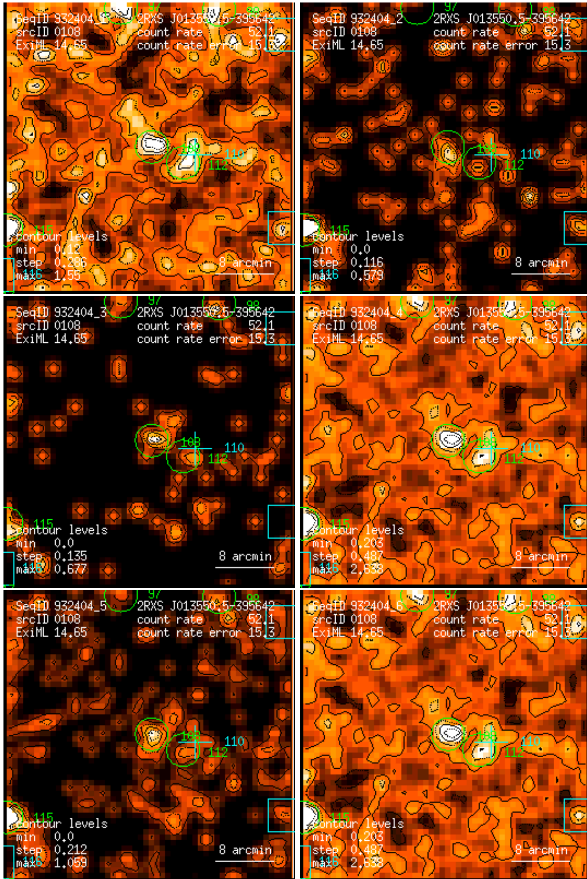
Figure 108: RASS 932404: detection 0108: band rate images, Gaussian filter: (1) PSPC channels 11 – 41, (2) 52 – 90, (3) 91 – 201, (4) 11 – 235, (5) 52 – 201, (6) 11 – 201. Broad band rates in counts/ks. Band rate contour levels in counts/ks/arcmin 2 .
