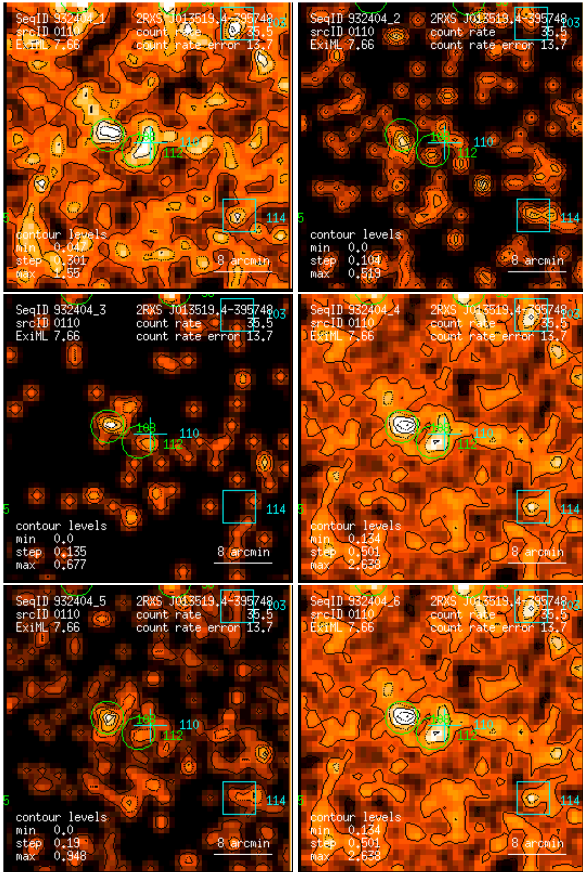
Figure 110: RASS 932404: detection 0110: band rate images, Gaussian filter: (1) PSPC channels 11 – 41, (2) 52 – 90, (3) 91 – 201, (4) 11 – 235, (5) 52 – 201, (6) 11 – 201. Broad band rates in counts/ks. Band rate contour levels in counts/ks/arcmin 2 .
