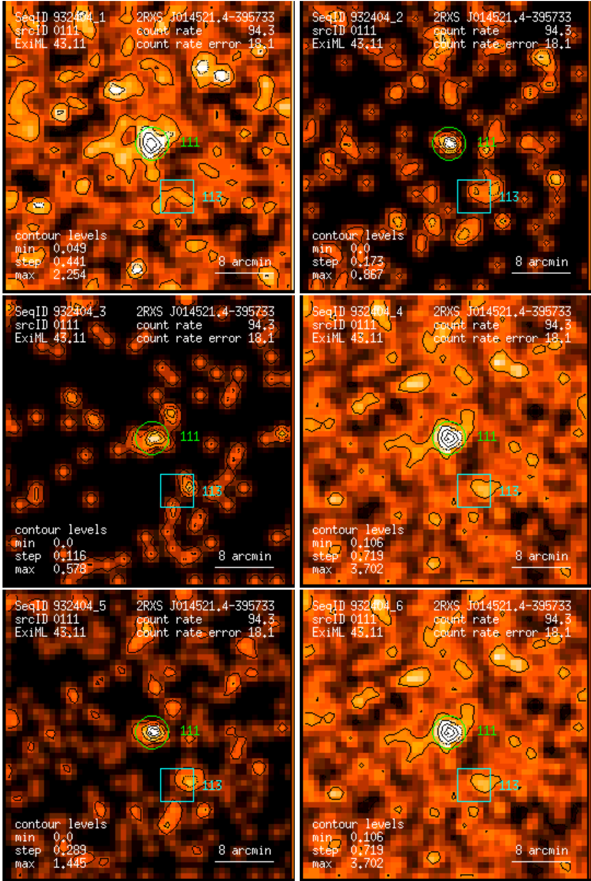
Figure 111: RASS 932404: detection 0111: band rate images, Gaussian filter: (1) PSPC channels 11 – 41, (2) 52 – 90, (3) 91 – 201, (4) 11 – 235, (5) 52 – 201, (6) 11 – 201. Broad band rates in counts/ks. Band rate contour levels in counts/ks/arcmin 2 .
