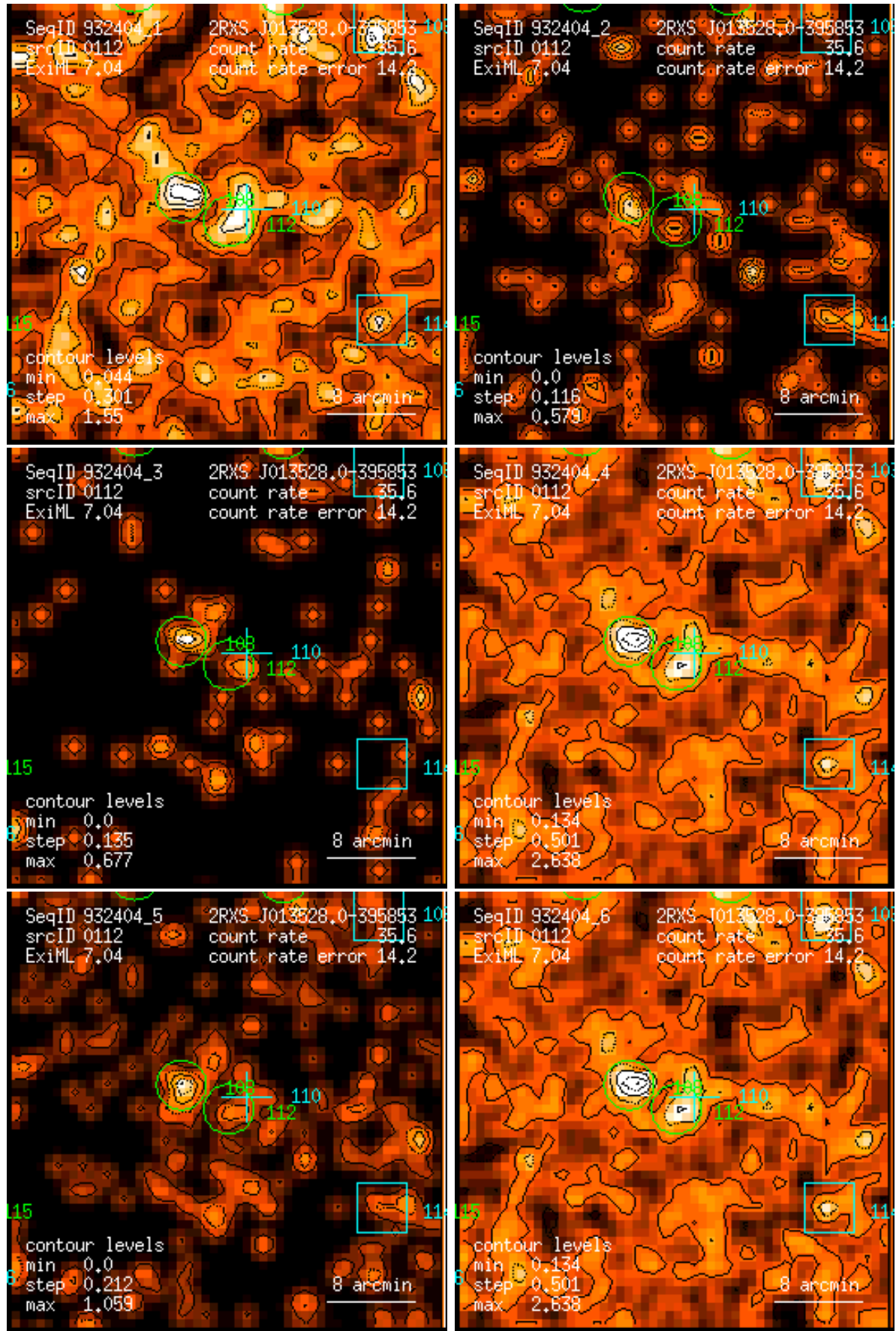
Figure 112: RASS 932404: detection 0112: band rate images, Gaussian filter: (1) PSPC channels 11 – 41, (2) 52 – 90, (3) 91 – 201, (4) 11 – 235, (5) 52 – 201, (6) 11 – 201. Broad band rates in counts/ks. Band rate contour levels in counts/ks/arcmin 2 .
