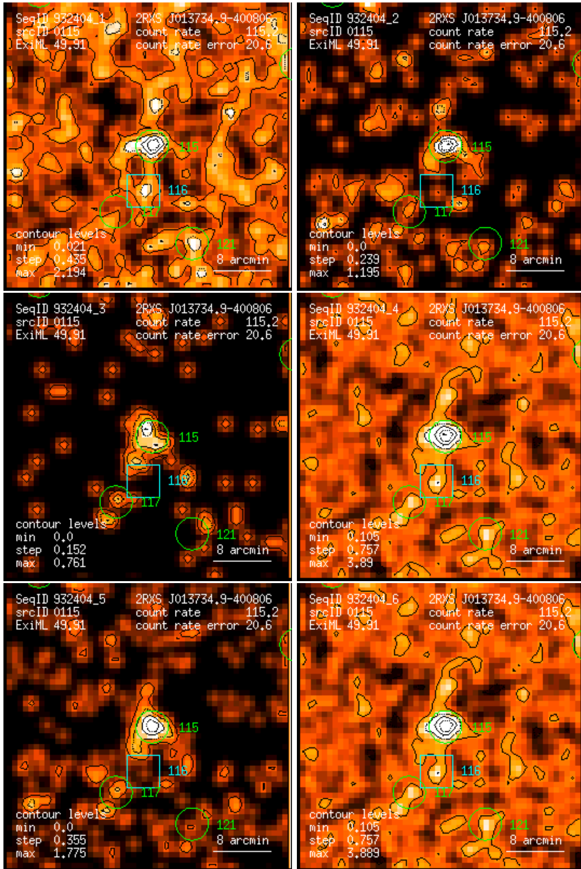
Figure 115: RASS 932404: detection 0115: band rate images, Gaussian filter: (1) PSPC channels 11 – 41, (2) 52 – 90, (3) 91 – 201, (4) 11 – 235, (5) 52 – 201, (6) 11 – 201. Broad band rates in counts/ks. Band rate contour levels in counts/ks/arcmin 2 .
