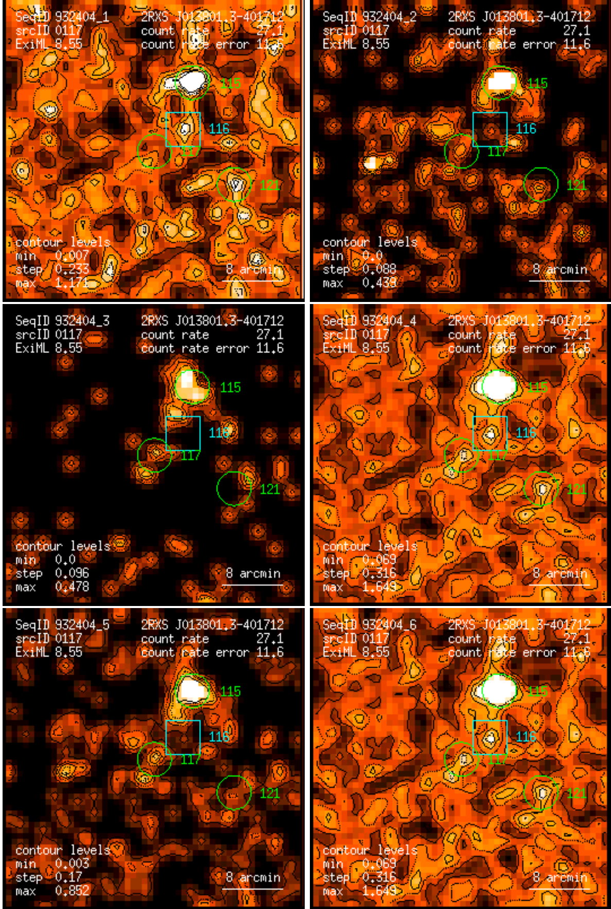
Figure 117: RASS 932404: detection 0117: band rate images, Gaussian filter: (1) PSPC channels 11 – 41, (2) 52 – 90, (3) 91 – 201, (4) 11 – 235, (5) 52 – 201, (6) 11 – 201. Broad band rates in counts/ks. Band rate contour levels in counts/ks/arcmin 2 .
