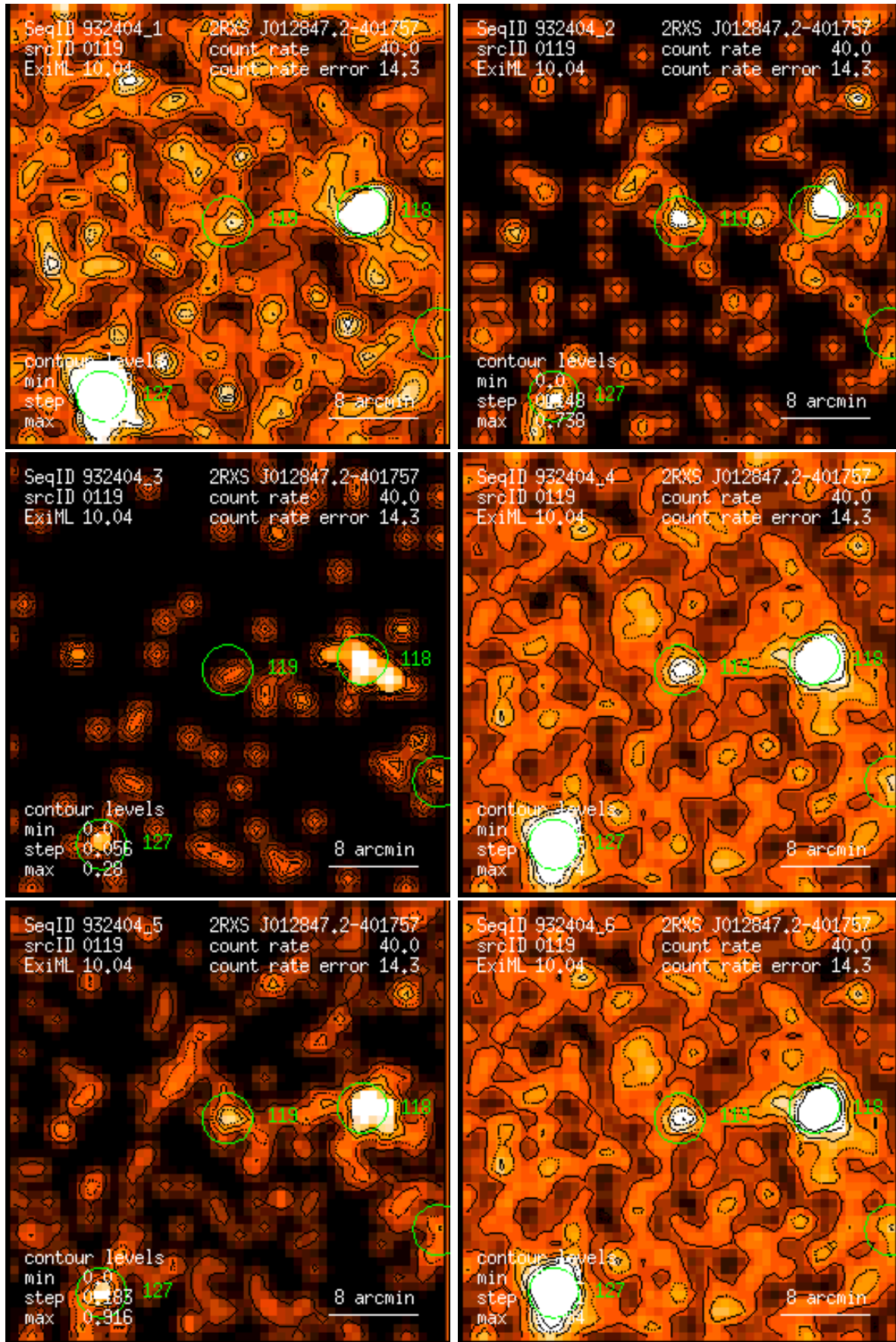
Figure 119: RASS 932404: detection 0119: band rate images, Gaussian filter: (1) PSPC channels 11 – 41, (2) 52 – 90, (3) 91 – 201, (4) 11 – 235, (5) 52 – 201, (6) 11 – 201. Broad band rates in counts/ks. Band rate contour levels in counts/ks/arcmin 2 .
