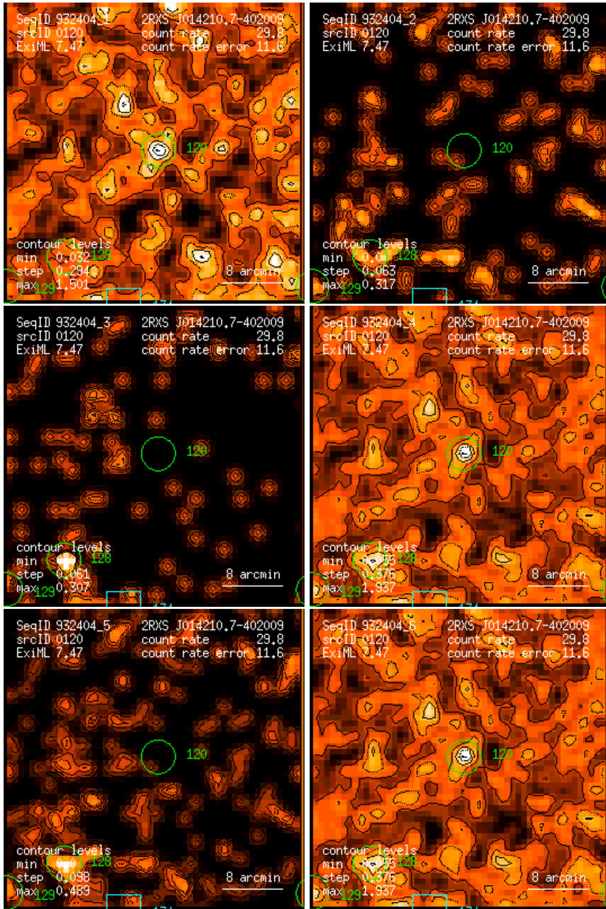
Figure 120: RASS 932404: detection 0120: band rate images, Gaussian filter: (1) PSPC channels 11 – 41, (2) 52 – 90, (3) 91 – 201, (4) 11 – 235, (5) 52 – 201, (6) 11 – 201. Broad band rates in counts/ks. Band rate contour levels in counts/ks/arcmin 2 .
