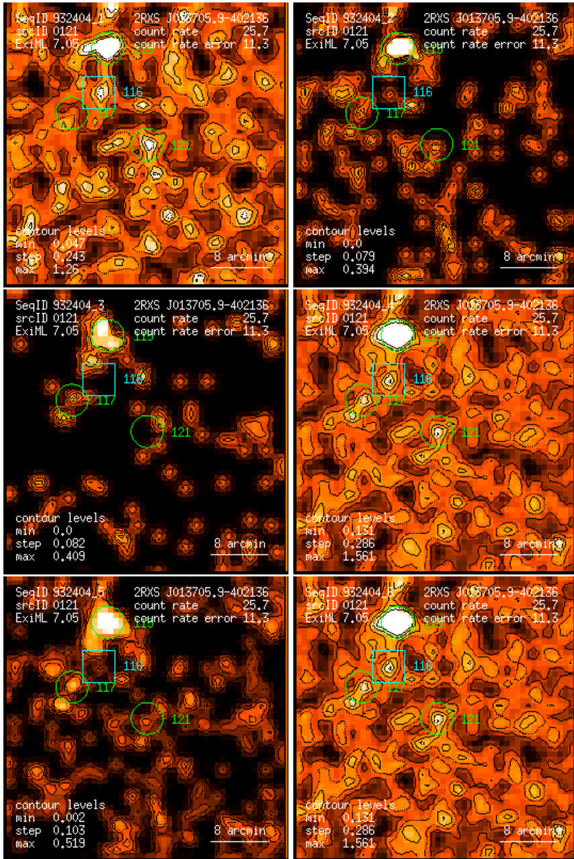
Figure 121: RASS 932404: detection 0121: band rate images, Gaussian filter: (1) PSPC channels 11 – 41, (2) 52 – 90, (3) 91 – 201, (4) 11 – 235, (5) 52 – 201, (6) 11 – 201. Broad band rates in counts/ks. Band rate contour levels in counts/ks/arcmin 2 .
