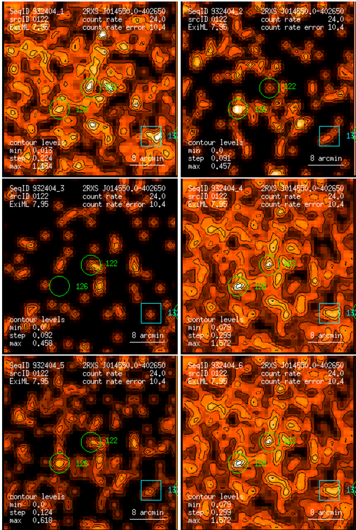
Figure 122: RASS 932404: detection 0122: band rate images, Gaussian filter: (1) PSPC channels 11 – 41, (2) 52 – 90, (3) 91 – 201, (4) 11 – 235, (5) 52 – 201, (6) 11 – 201. Broad band rates in counts/ks. Band rate contour levels in counts/ks/arcmin 2 .
