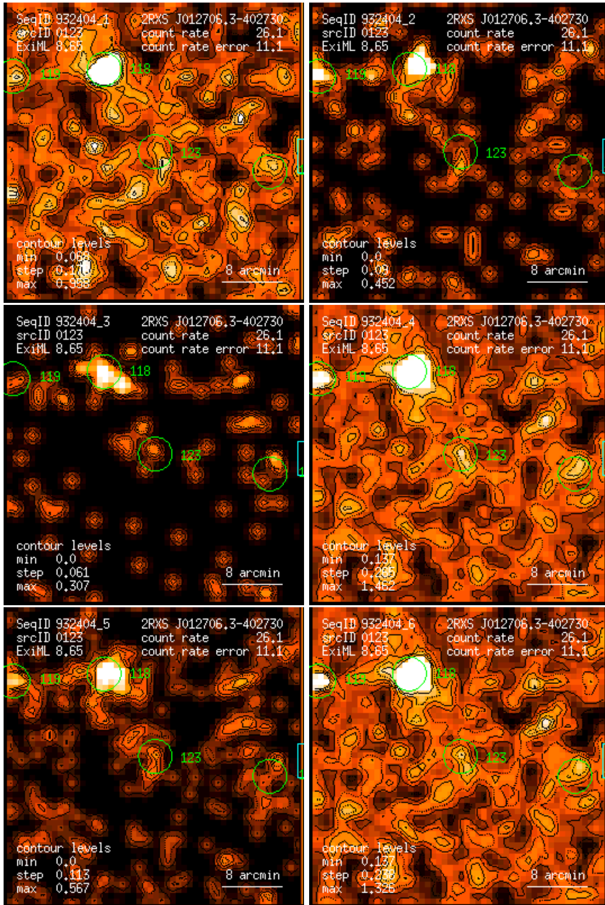
Figure 123: RASS 932404: detection 0123: band rate images, Gaussian filter: (1) PSPC channels 11 – 41, (2) 52 – 90, (3) 91 – 201, (4) 11 – 235, (5) 52 – 201, (6) 11 – 201. Broad band rates in counts/ks. Band rate contour levels in counts/ks/arcmin 2 .
