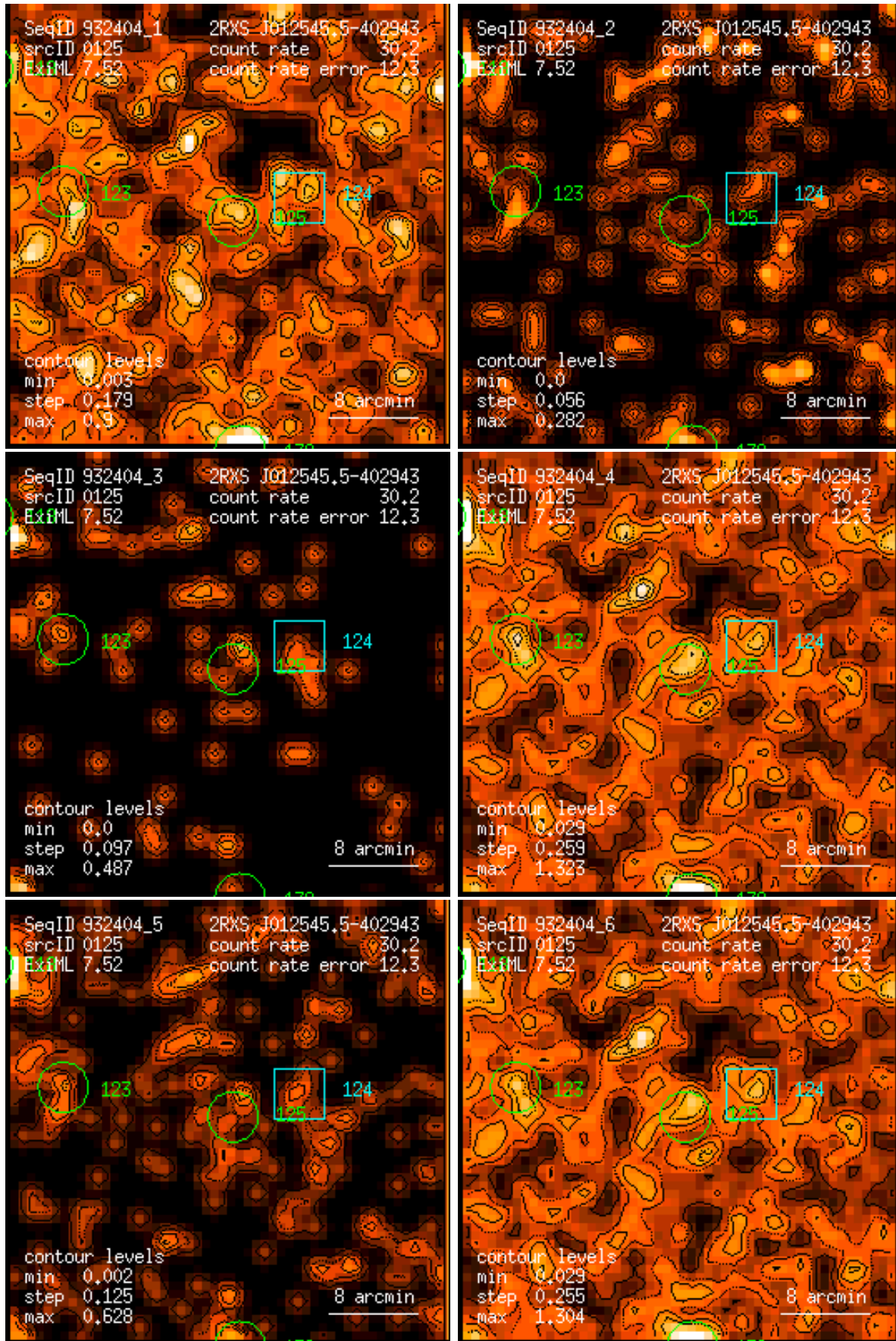
Figure 125: RASS 932404: detection 0125: band rate images, Gaussian filter: (1) PSPC channels 11 – 41, (2) 52 – 90, (3) 91 – 201, (4) 11 – 235, (5) 52 – 201, (6) 11 – 201. Broad band rates in counts/ks. Band rate contour levels in counts/ks/arcmin 2 .
