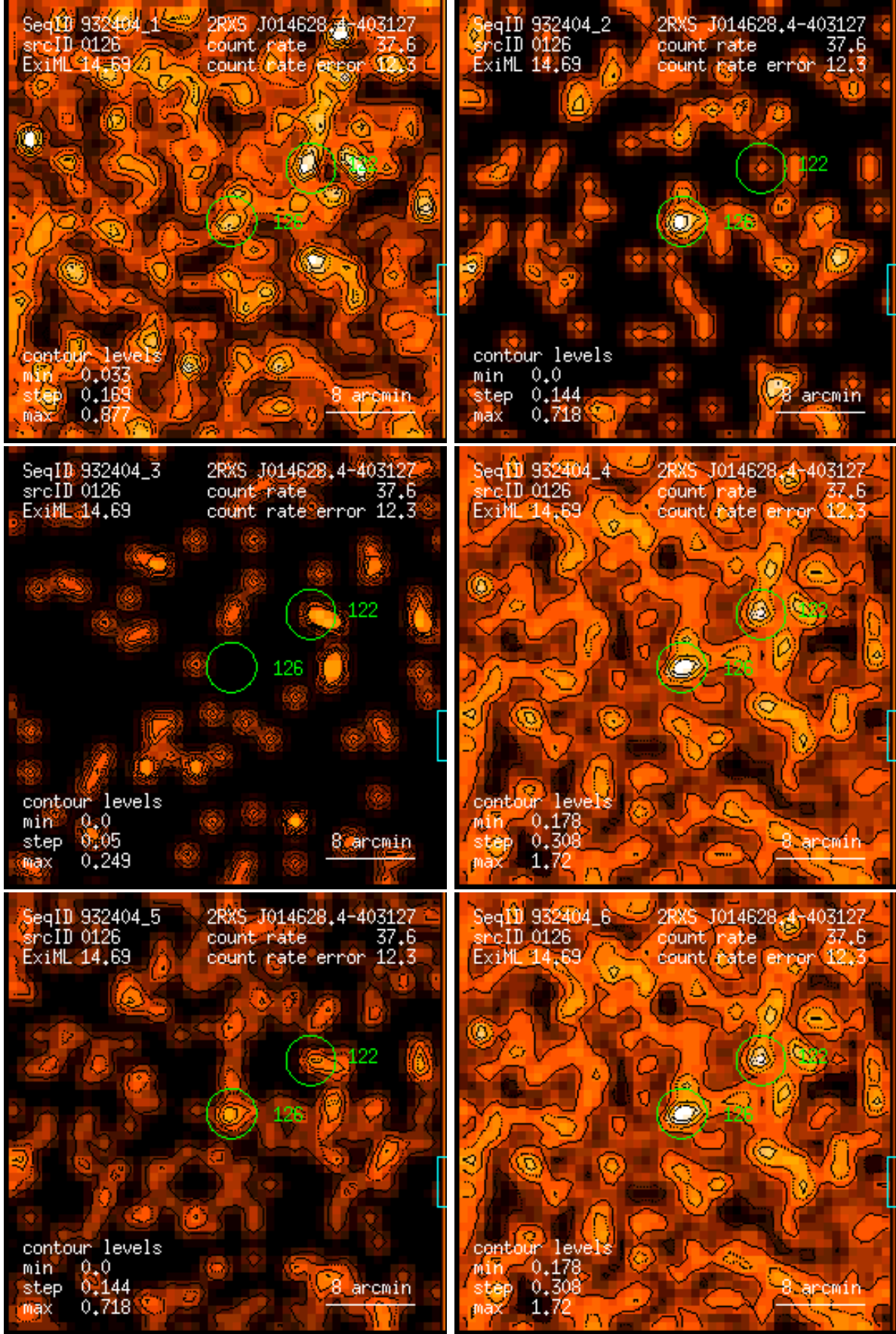
Figure 126: RASS 932404: detection 0126: band rate images, Gaussian filter: (1) PSPC channels 11 – 41, (2) 52 – 90, (3) 91 – 201, (4) 11 – 235, (5) 52 – 201, (6) 11 – 201. Broad band rates in counts/ks. Band rate contour levels in counts/ks/arcmin 2 .
