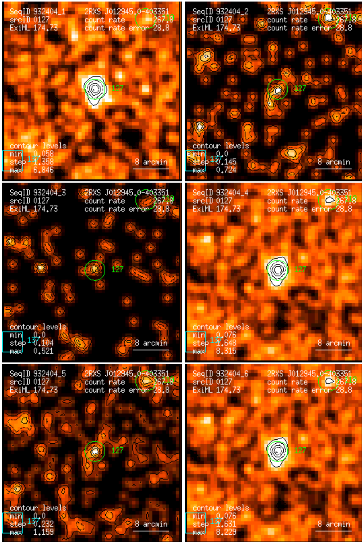
Figure 127: RASS 932404: detection 0127: band rate images, Gaussian filter: (1) PSPC channels 11 – 41, (2) 52 – 90, (3) 91 – 201, (4) 11 – 235, (5) 52 – 201, (6) 11 – 201. Broad band rates in counts/ks. Band rate contour levels in counts/ks/arcmin 2 .
