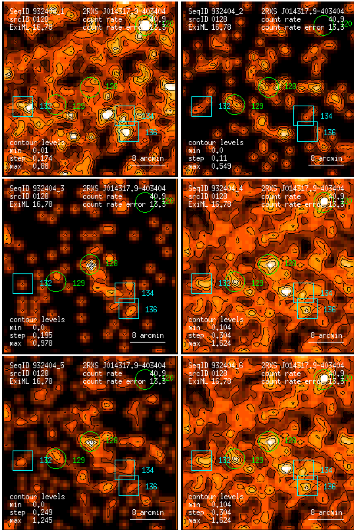
Figure 128: RASS 932404: detection 0128: band rate images, Gaussian filter: (1) PSPC channels 11 – 41, (2) 52 – 90, (3) 91 – 201, (4) 11 – 235, (5) 52 – 201, (6) 11 – 201. Broad band rates in counts/ks. Band rate contour levels in counts/ks/arcmin 2 .
