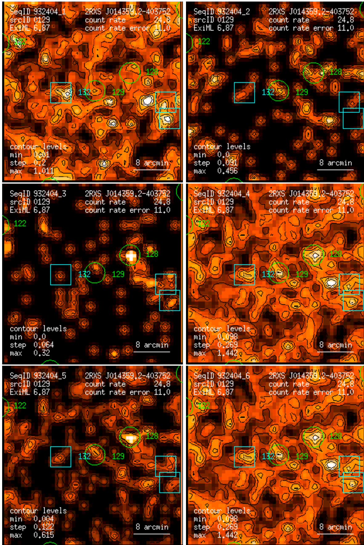
Figure 129: RASS 932404: detection 0129: band rate images, Gaussian filter: (1) PSPC channels 11 – 41, (2) 52 – 90, (3) 91 – 201, (4) 11 – 235, (5) 52 – 201, (6) 11 – 201. Broad band rates in counts/ks. Band rate contour levels in counts/ks/arcmin 2 .
