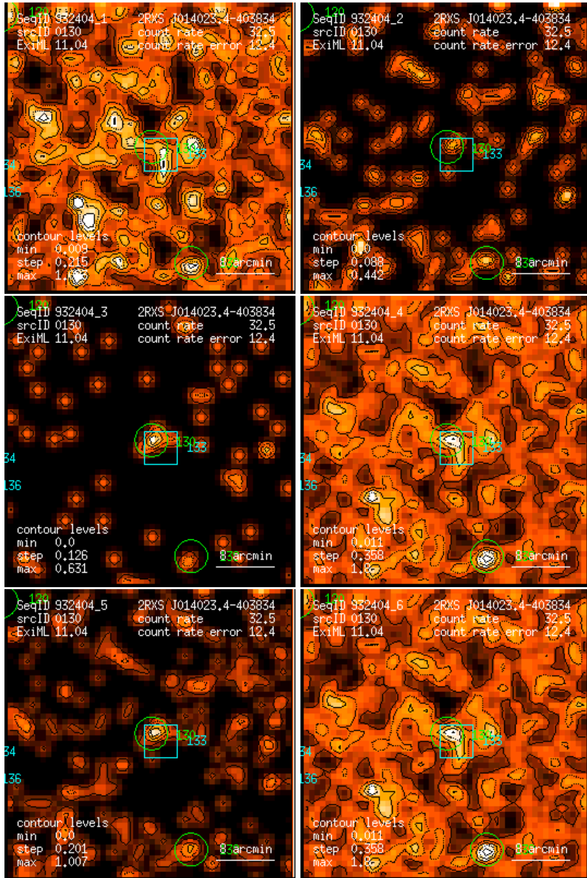
Figure 130: RASS 932404: detection 0130: band rate images, Gaussian filter: (1) PSPC channels 11 – 41, (2) 52 – 90, (3) 91 – 201, (4) 11 – 235, (5) 52 – 201, (6) 11 – 201. Broad band rates in counts/ks. Band rate contour levels in counts/ks/arcmin 2 .
