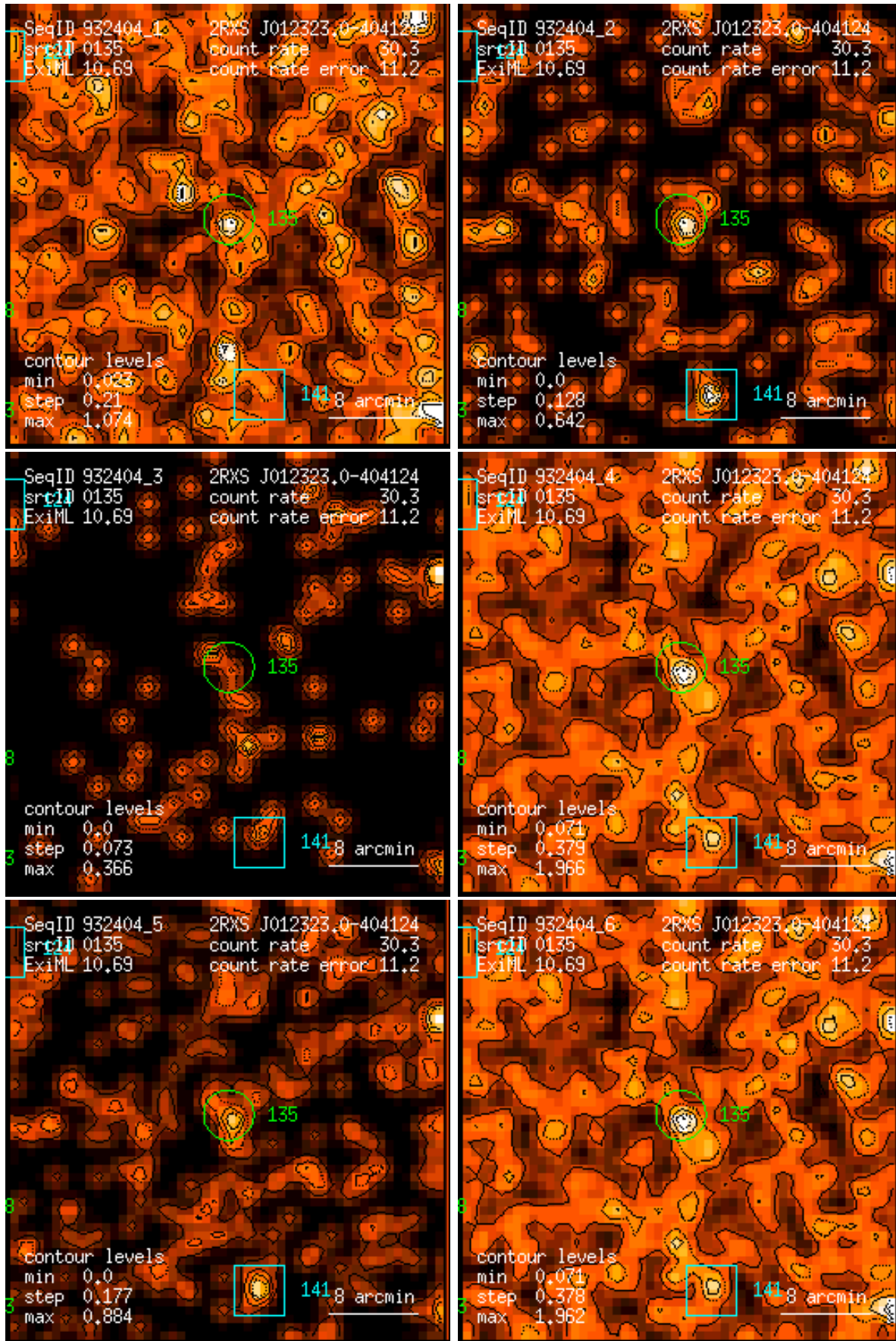
Figure 135: RASS 932404: detection 0135: band rate images, Gaussian filter: (1) PSPC channels 11 – 41, (2) 52 – 90, (3) 91 – 201, (4) 11 – 235, (5) 52 – 201, (6) 11 – 201. Broad band rates in counts/ks. Band rate contour levels in counts/ks/arcmin 2 .
