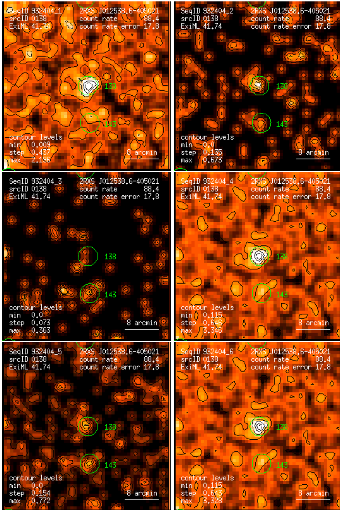
Figure 138: RASS 932404: detection 0138: band rate images, Gaussian filter: (1) PSPC channels 11 – 41, (2) 52 – 90, (3) 91 – 201, (4) 11 – 235, (5) 52 – 201, (6) 11 – 201. Broad band rates in counts/ks. Band rate contour levels in counts/ks/arcmin 2 .
