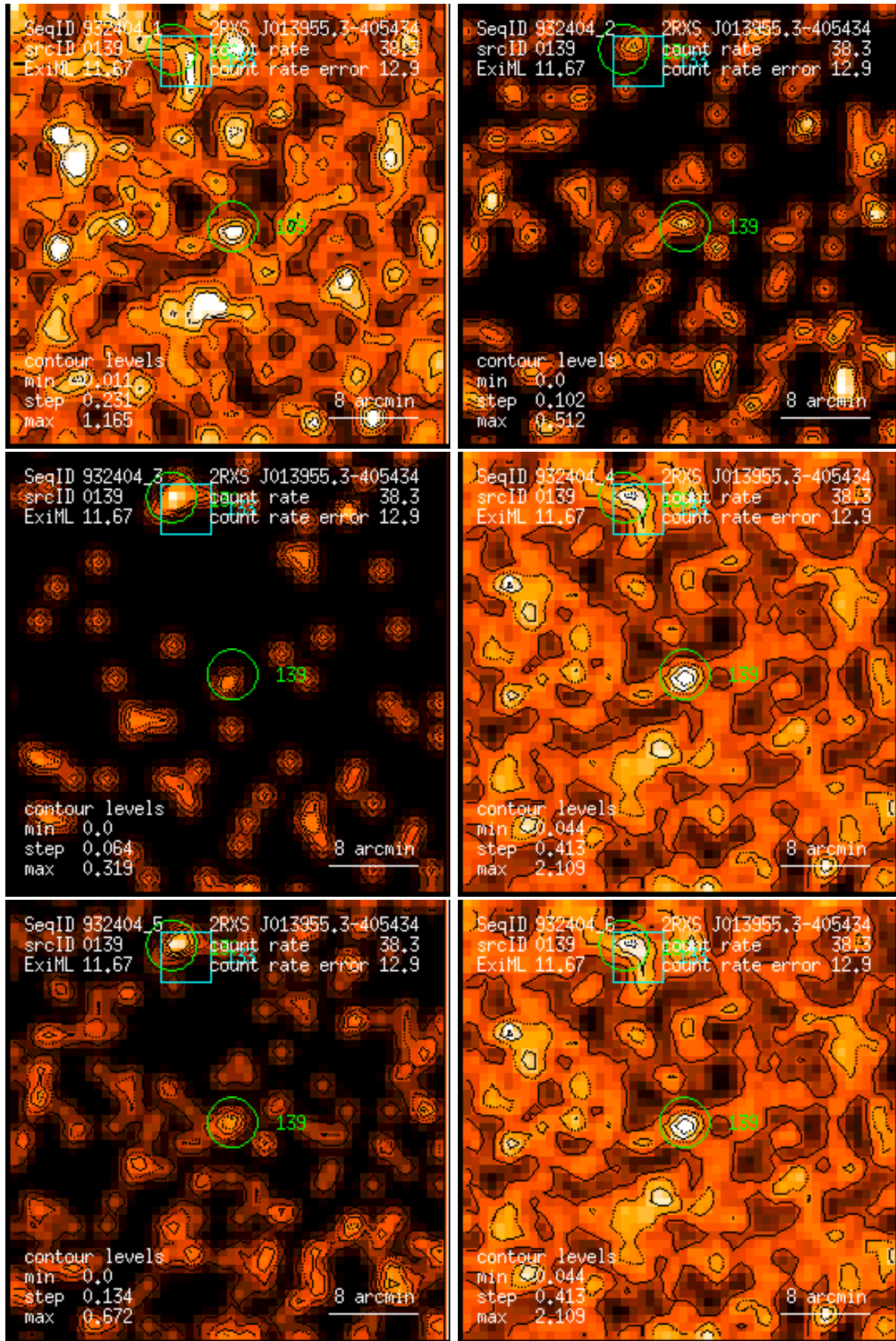
Figure 139: RASS 932404: detection 0139: band rate images, Gaussian filter: (1) PSPC channels 11 – 41, (2) 52 – 90, (3) 91 – 201, (4) 11 – 235, (5) 52 – 201, (6) 11 – 201. Broad band rates in counts/ks. Band rate contour levels in counts/ks/arcmin 2 .
