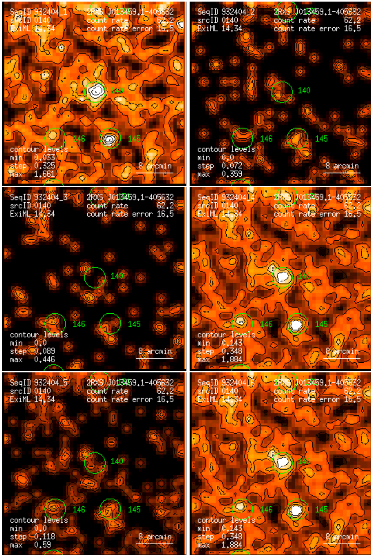
Figure 140: RASS 932404: detection 0140: band rate images, Gaussian filter: (1) PSPC channels 11 – 41, (2) 52 – 90, (3) 91 – 201, (4) 11 – 235, (5) 52 – 201, (6) 11 – 201. Broad band rates in counts/ks. Band rate contour levels in counts/ks/arcmin 2 .
