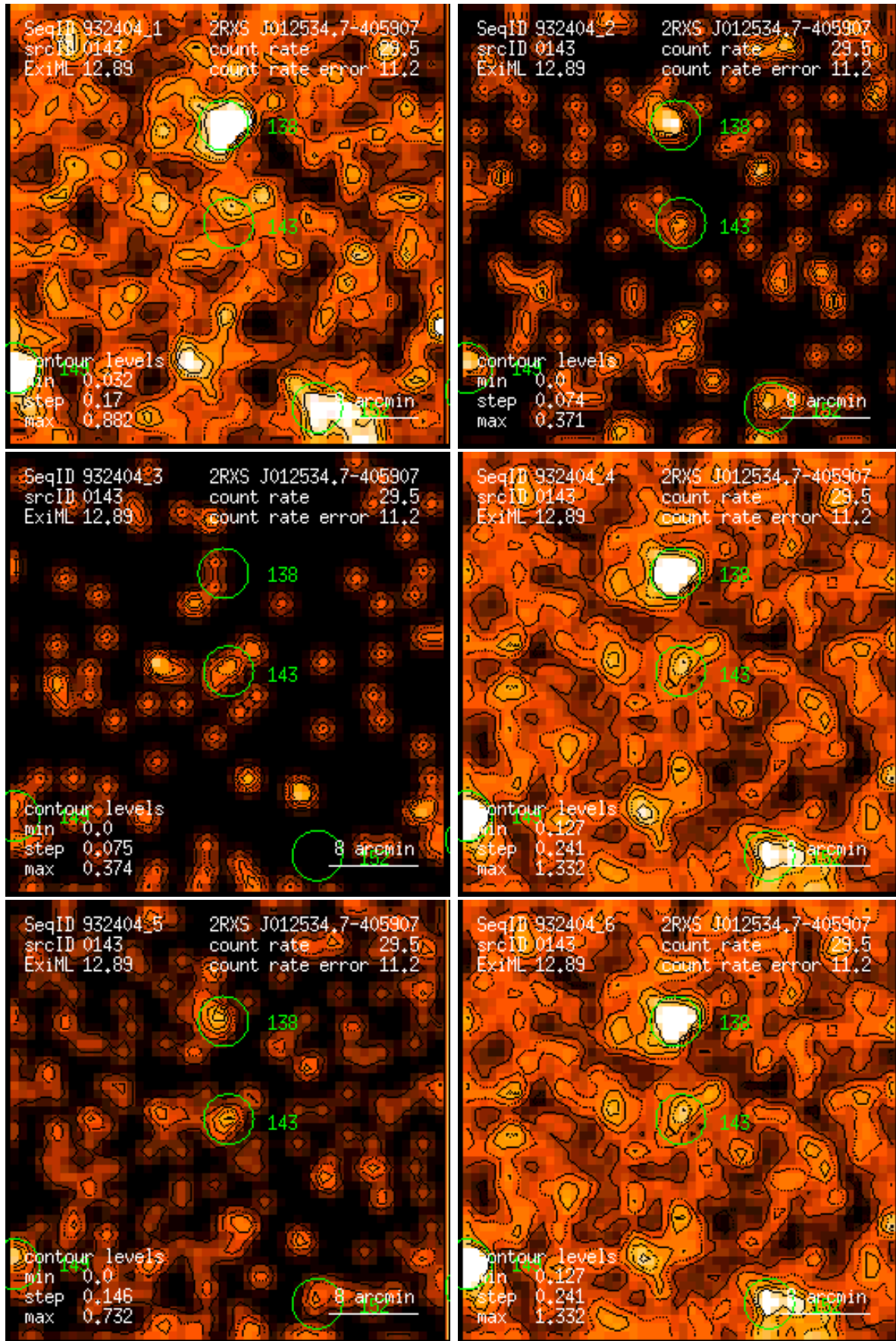
Figure 143: RASS 932404: detection 0143: band rate images, Gaussian filter: (1) PSPC channels 11 – 41, (2) 52 – 90, (3) 91 – 201, (4) 11 – 235, (5) 52 – 201, (6) 11 – 201. Broad band rates in counts/ks. Band rate contour levels in counts/ks/arcmin 2 .
