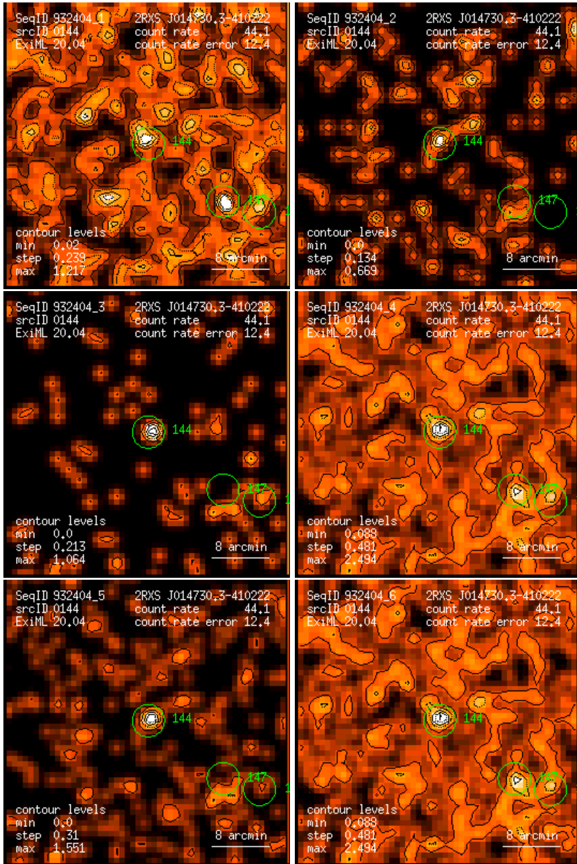
Figure 144: RASS 932404: detection 0144: band rate images, Gaussian filter: (1) PSPC channels 11 – 41, (2) 52 – 90, (3) 91 – 201, (4) 11 – 235, (5) 52 – 201, (6) 11 – 201. Broad band rates in counts/ks. Band rate contour levels in counts/ks/arcmin 2 .
