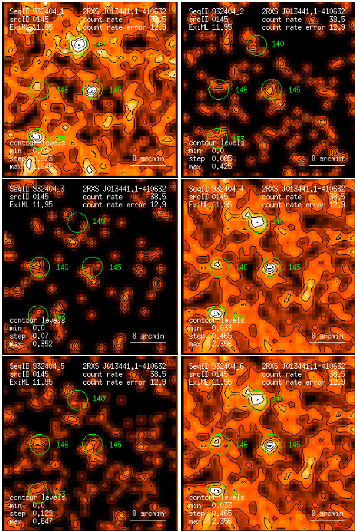
Figure 145: RASS 932404: detection 0145: band rate images, Gaussian filter: (1) PSPC channels 11 – 41, (2) 52 – 90, (3) 91 – 201, (4) 11 – 235, (5) 52 – 201, (6) 11 – 201. Broad band rates in counts/ks. Band rate contour levels in counts/ks/arcmin 2 .
