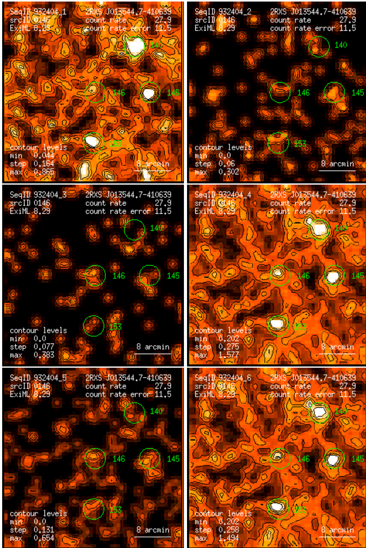
Figure 146: RASS 932404: detection 0146: band rate images, Gaussian filter: (1) PSPC channels 11 – 41, (2) 52 – 90, (3) 91 – 201, (4) 11 – 235, (5) 52 – 201, (6) 11 – 201. Broad band rates in counts/ks. Band rate contour levels in counts/ks/arcmin 2 .
