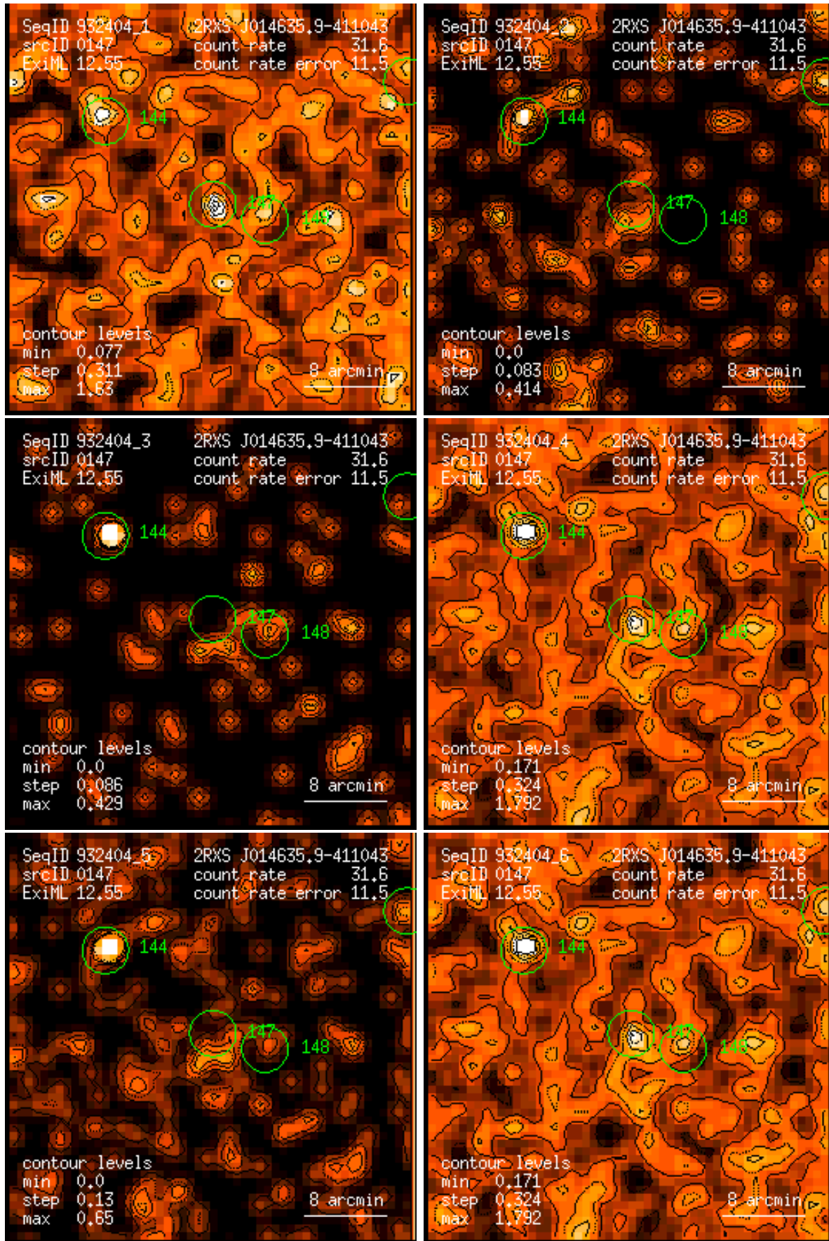
Figure 147: RASS 932404: detection 0147: band rate images, Gaussian filter: (1) PSPC channels 11 – 41, (2) 52 – 90, (3) 91 – 201, (4) 11 – 235, (5) 52 – 201, (6) 11 – 201. Broad band rates in counts/ks. Band rate contour levels in counts/ks/arcmin 2 .
