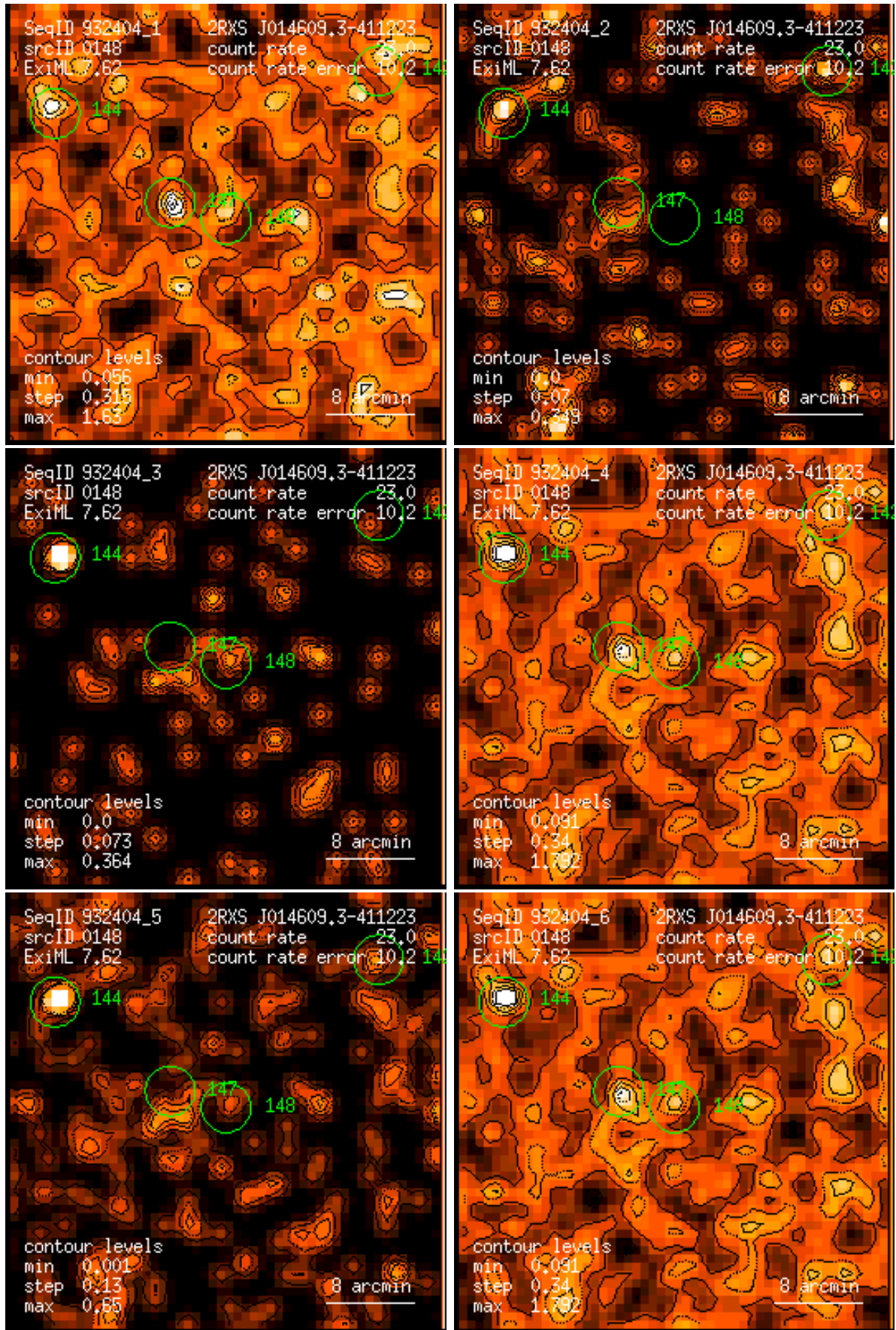
Figure 148: RASS 932404: detection 0148: band rate images, Gaussian filter: (1) PSPC channels 11 – 41, (2) 52 – 90, (3) 91 – 201, (4) 11 – 235, (5) 52 – 201, (6) 11 – 201. Broad band rates in counts/ks. Band rate contour levels in counts/ks/arcmin 2 .
