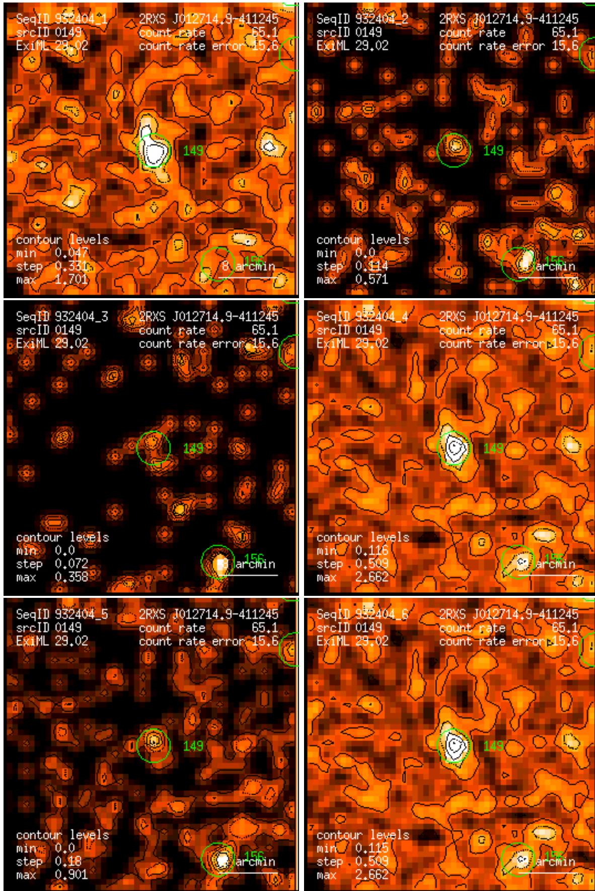
Figure 149: RASS 932404: detection 0149: band rate images, Gaussian filter: (1) PSPC channels 11 – 41, (2) 52 – 90, (3) 91 – 201, (4) 11 – 235, (5) 52 – 201, (6) 11 – 201. Broad band rates in counts/ks. Band rate contour levels in counts/ks/arcmin 2 .
