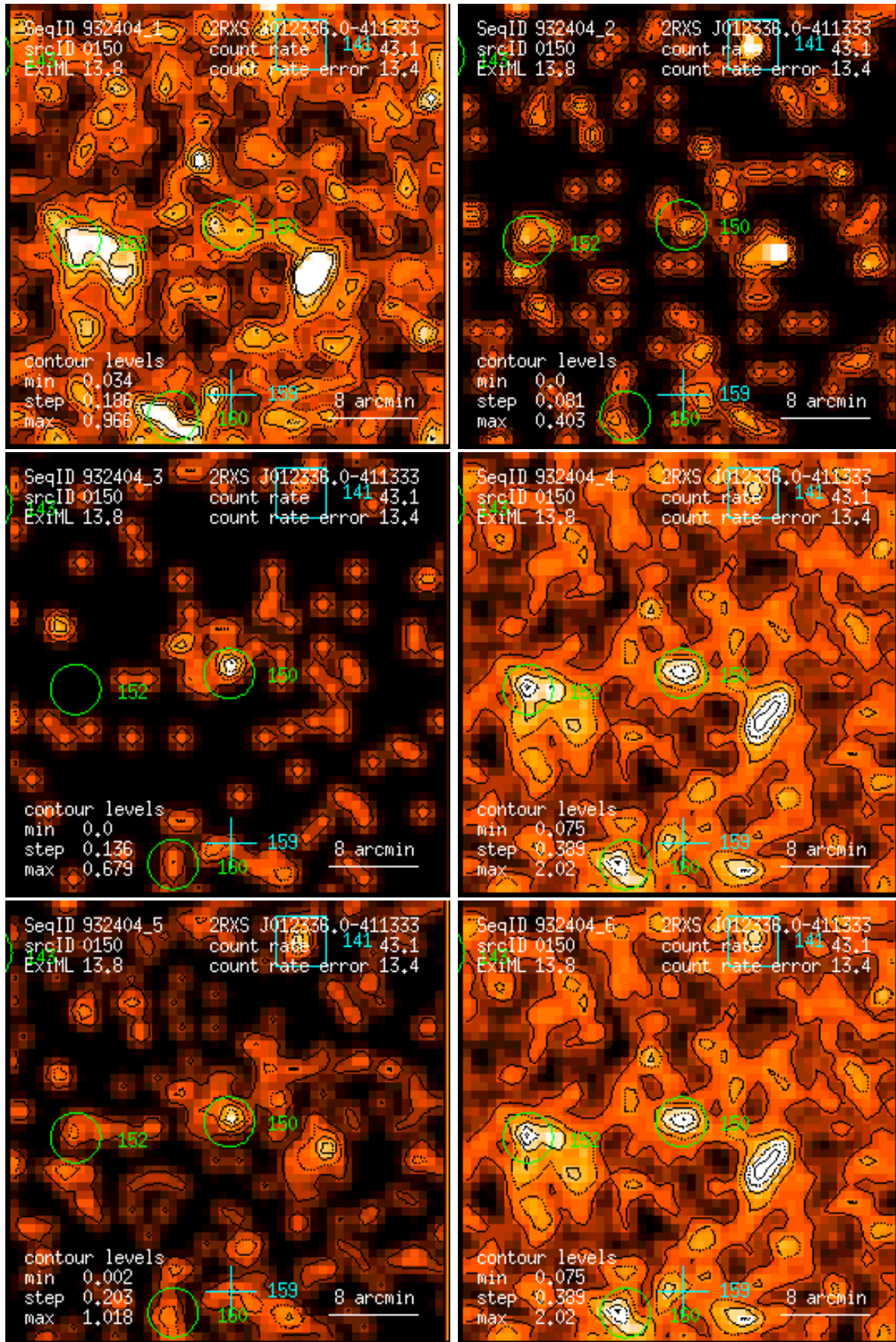
Figure 150: RASS 932404: detection 0150: band rate images, Gaussian filter: (1) PSPC channels 11 – 41, (2) 52 – 90, (3) 91 – 201, (4) 11 – 235, (5) 52 – 201, (6) 11 – 201. Broad band rates in counts/ks. Band rate contour levels in counts/ks/arcmin 2 .
