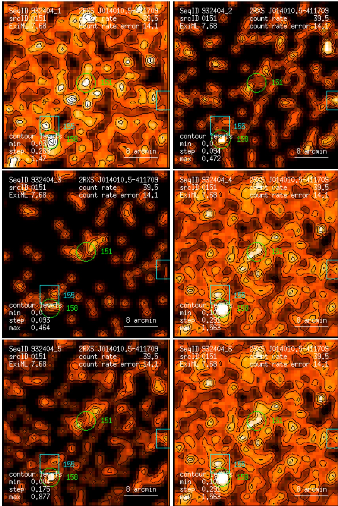
Figure 151: RASS 932404: detection 0151: band rate images, Gaussian filter: (1) PSPC channels 11 – 41, (2) 52 – 90, (3) 91 – 201, (4) 11 – 235, (5) 52 – 201, (6) 11 – 201. Broad band rates in counts/ks. Band rate contour levels in counts/ks/arcmin 2 .
