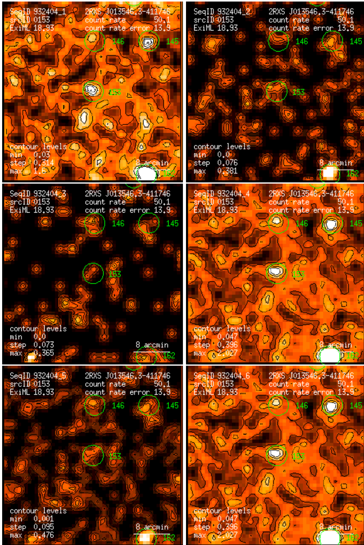
Figure 153: RASS 932404: detection 0153: band rate images, Gaussian filter: (1) PSPC channels 11 – 41, (2) 52 – 90, (3) 91 – 201, (4) 11 – 235, (5) 52 – 201, (6) 11 – 201. Broad band rates in counts/ks. Band rate contour levels in counts/ks/arcmin 2 .
