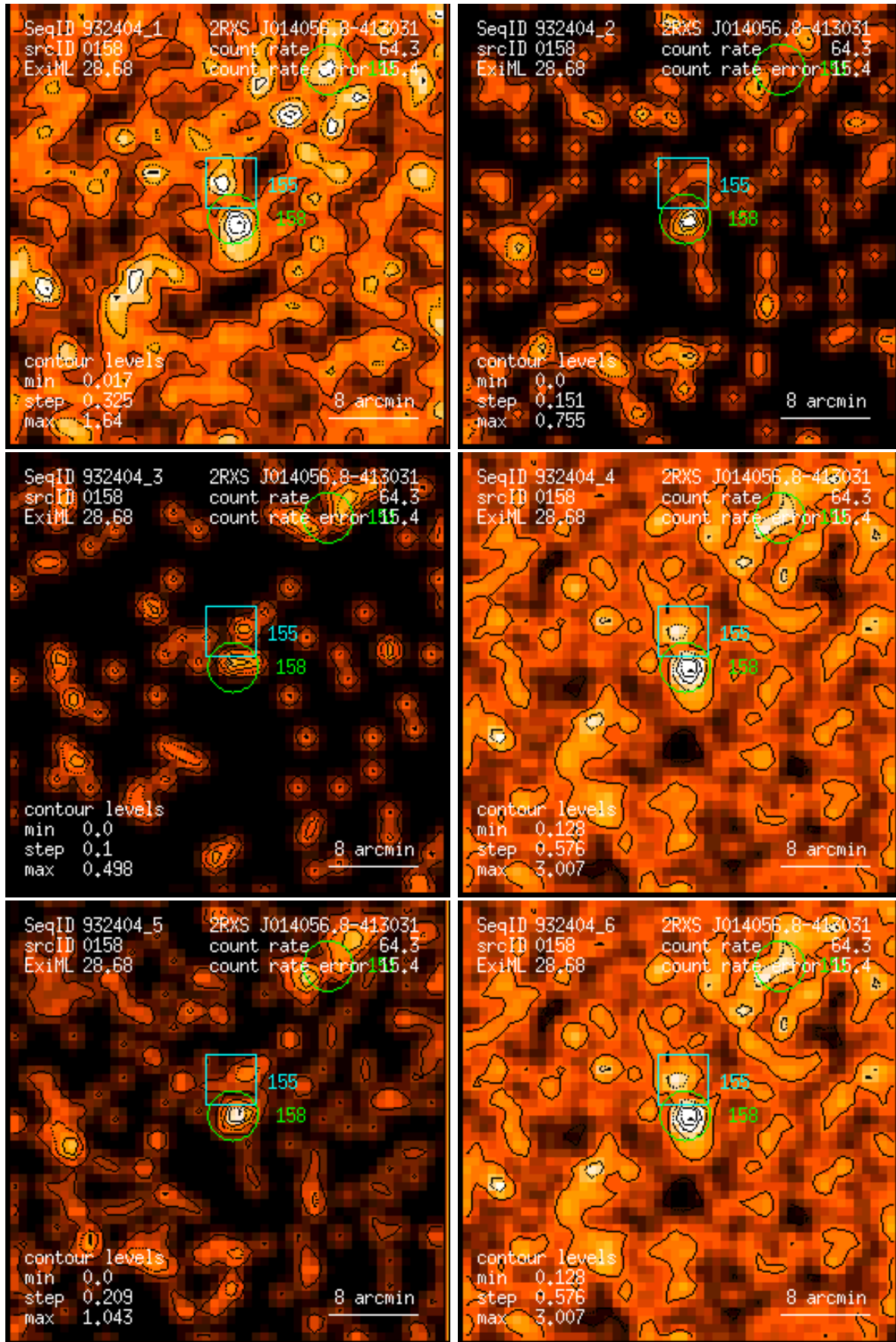
Figure 158: RASS 932404: detection 0158: band rate images, Gaussian filter: (1) PSPC channels 11 – 41, (2) 52 – 90, (3) 91 – 201, (4) 11 – 235, (5) 52 – 201, (6) 11 – 201. Broad band rates in counts/ks. Band rate contour levels in counts/ks/arcmin 2 .
