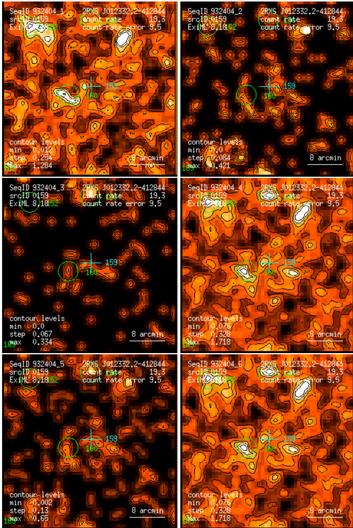
Figure 159: RASS 932404: detection 0159: band rate images, Gaussian filter: (1) PSPC channels 11 – 41, (2) 52 – 90, (3) 91 – 201, (4) 11 – 235, (5) 52 – 201, (6) 11 – 201. Broad band rates in counts/ks. Band rate contour levels in counts/ks/arcmin 2 .
