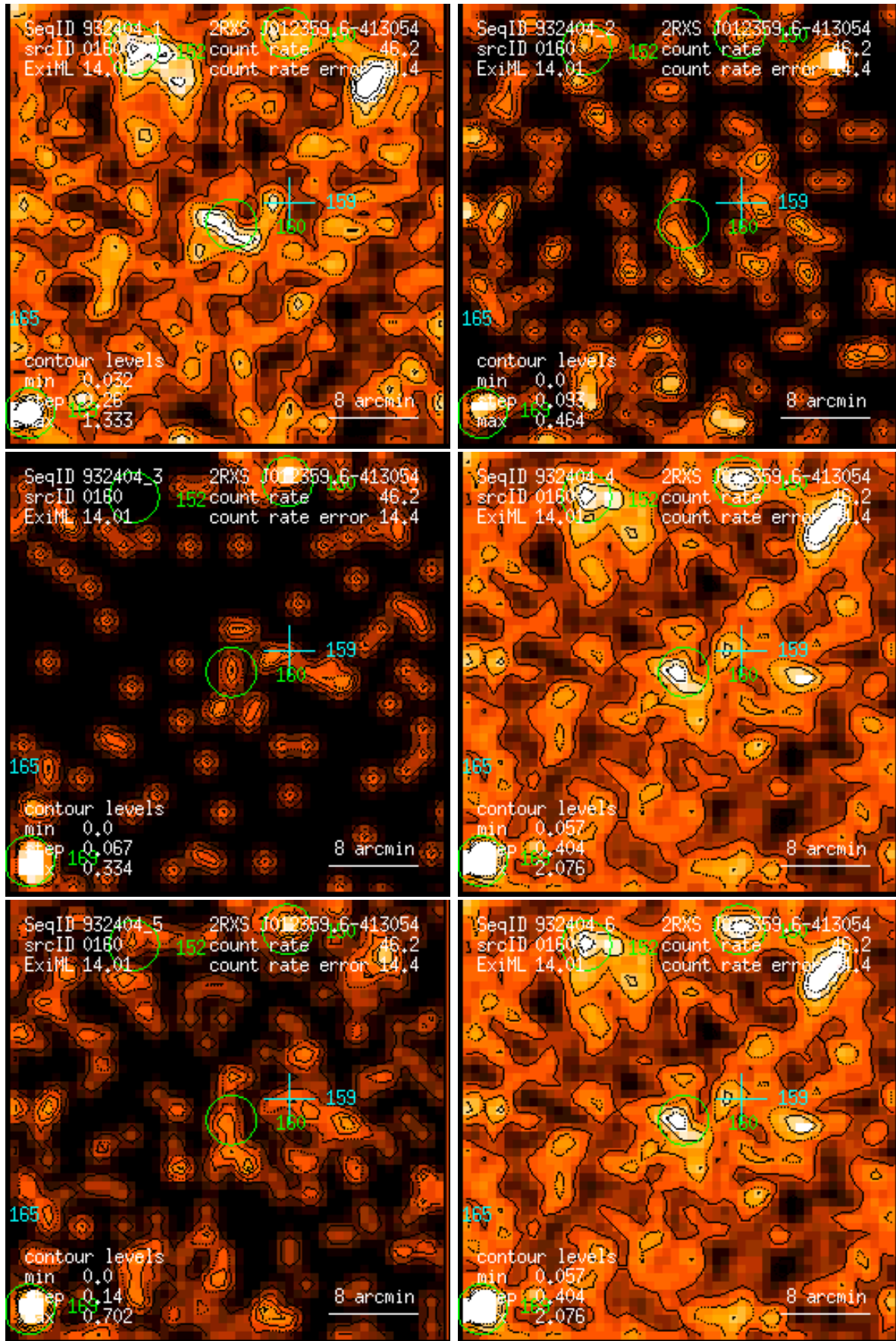
Figure 160: RASS 932404: detection 0160: band rate images, Gaussian filter: (1) PSPC channels 11 – 41, (2) 52 – 90, (3) 91 – 201, (4) 11 – 235, (5) 52 – 201, (6) 11 – 201. Broad band rates in counts/ks. Band rate contour levels in counts/ks/arcmin 2 .
