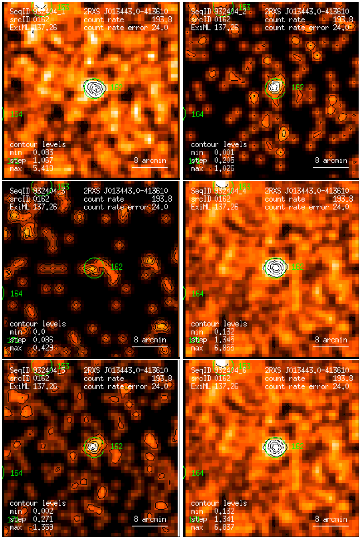
Figure 162: RASS 932404: detection 0162: band rate images, Gaussian filter: (1) PSPC channels 11 – 41, (2) 52 – 90, (3) 91 – 201, (4) 11 – 235, (5) 52 – 201, (6) 11 – 201. Broad band rates in counts/ks. Band rate contour levels in counts/ks/arcmin 2 .
