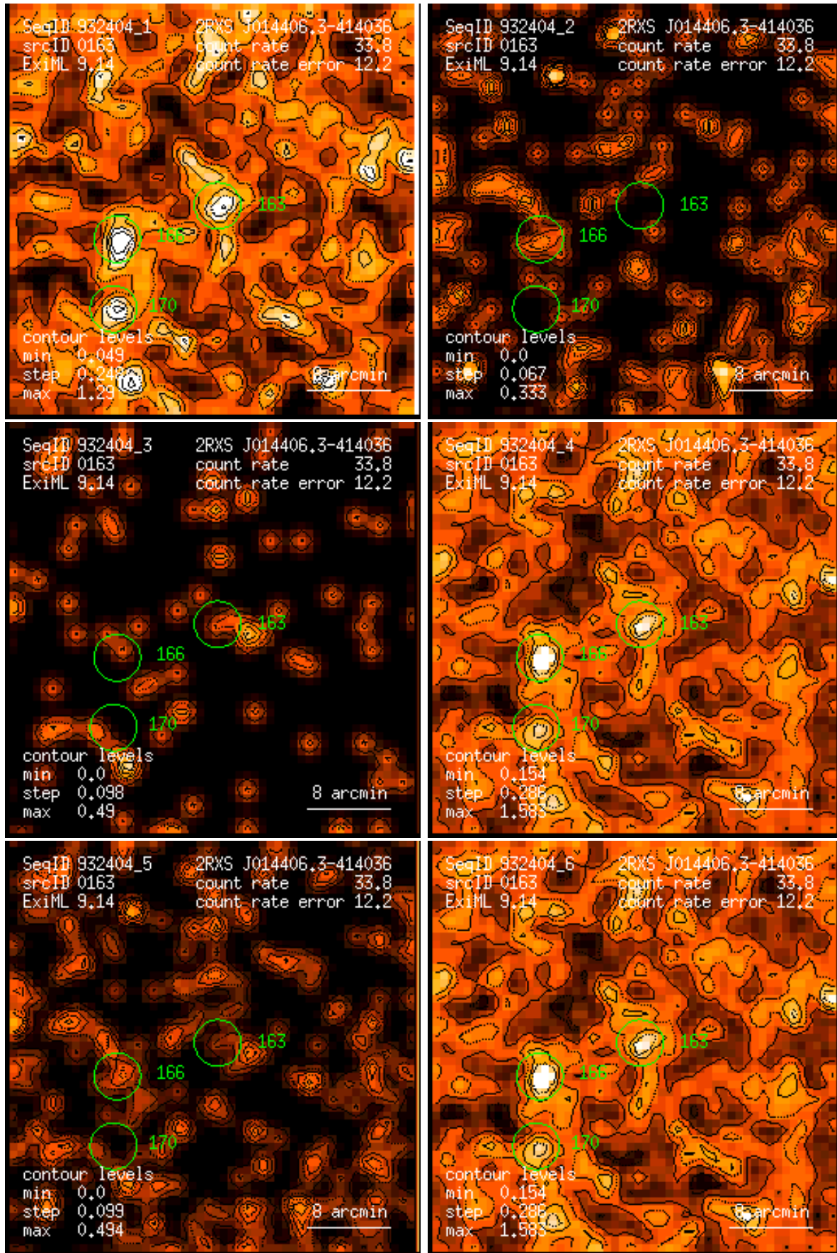
Figure 163: RASS 932404: detection 0163: band rate images, Gaussian filter: (1) PSPC channels 11 – 41, (2) 52 – 90, (3) 91 – 201, (4) 11 – 235, (5) 52 – 201, (6) 11 – 201. Broad band rates in counts/ks. Band rate contour levels in counts/ks/arcmin 2 .
