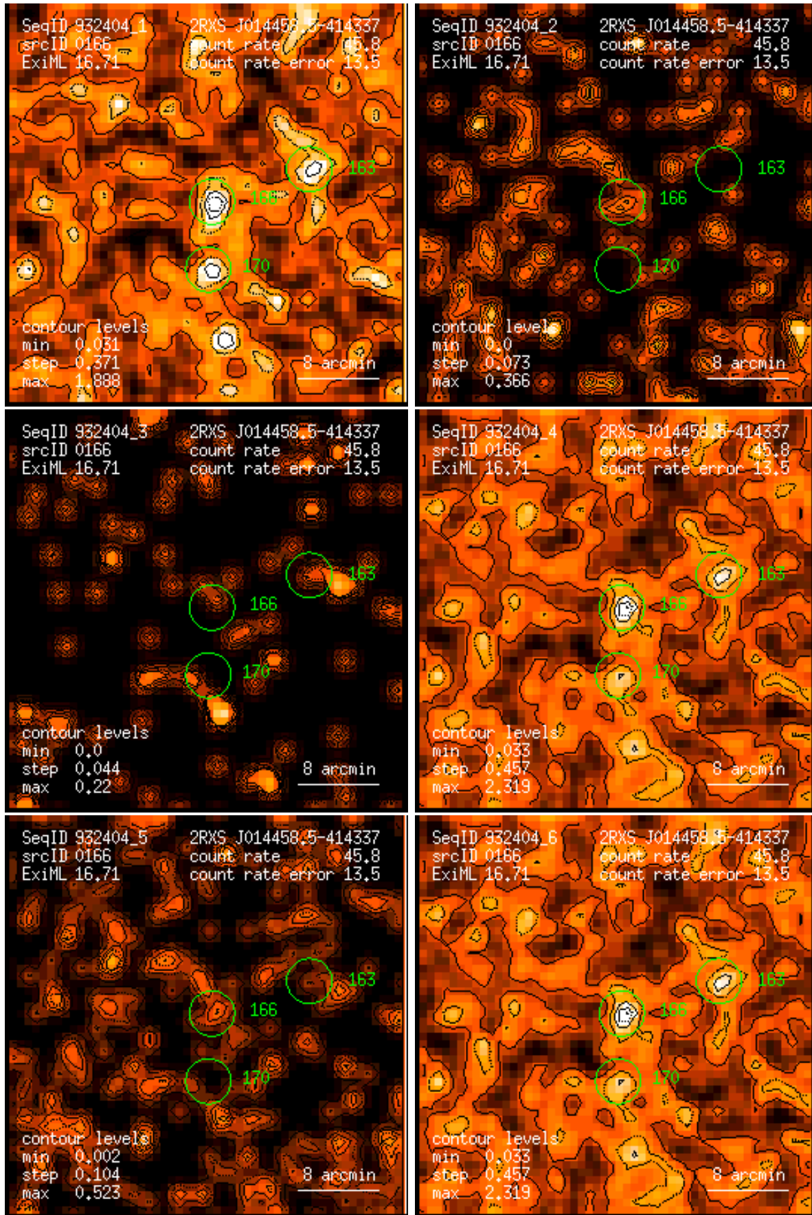
Figure 166: RASS 932404: detection 0166: band rate images, Gaussian filter: (1) PSPC channels 11 – 41, (2) 52 – 90, (3) 91 – 201, (4) 11 – 235, (5) 52 – 201, (6) 11 – 201. Broad band rates in counts/ks. Band rate contour levels in counts/ks/arcmin 2 .
