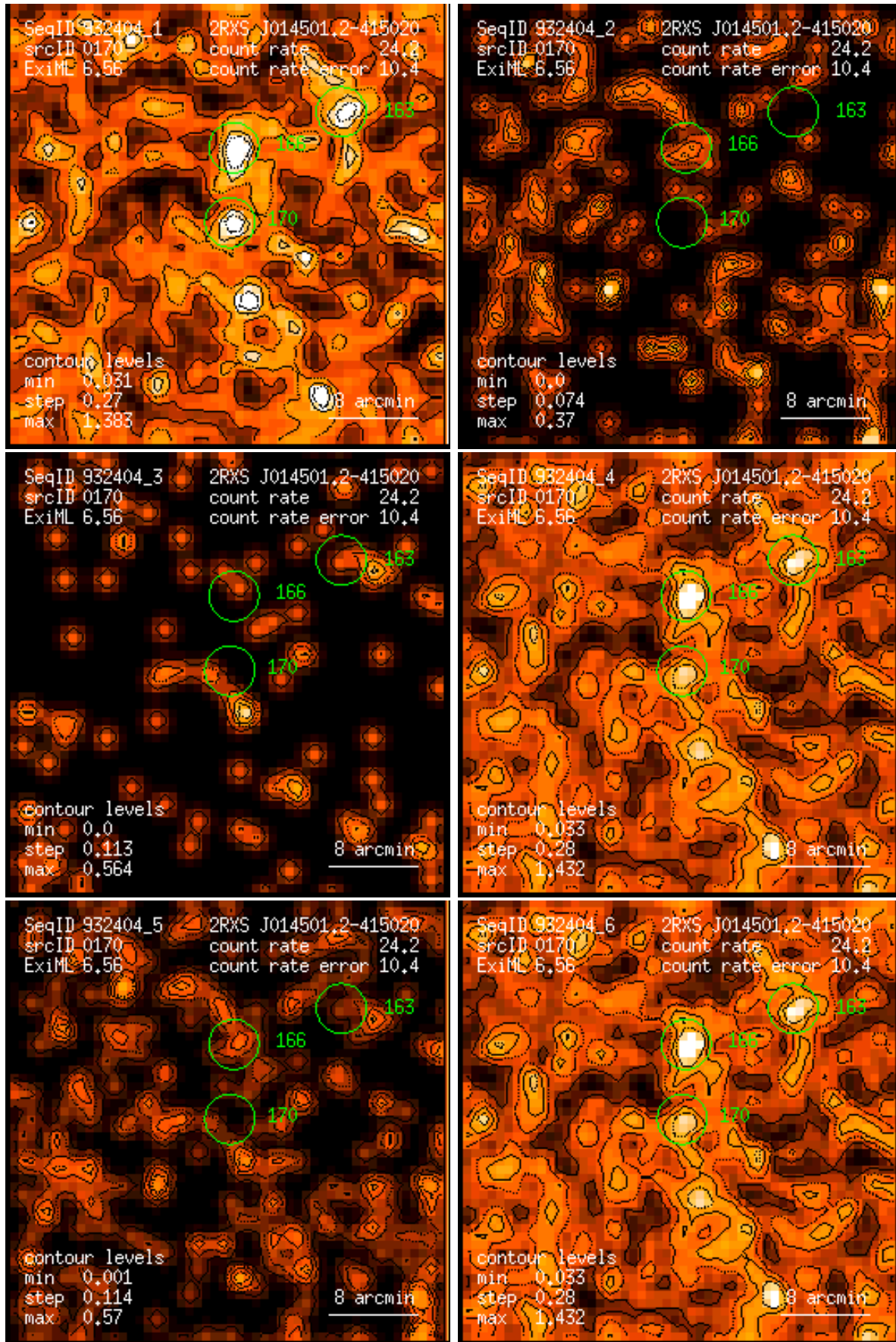
Figure 170: RASS 932404: detection 0170: band rate images, Gaussian filter: (1) PSPC channels 11 – 41, (2) 52 – 90, (3) 91 – 201, (4) 11 – 235, (5) 52 – 201, (6) 11 – 201. Broad band rates in counts/ks. Band rate contour levels in counts/ks/arcmin 2 .
