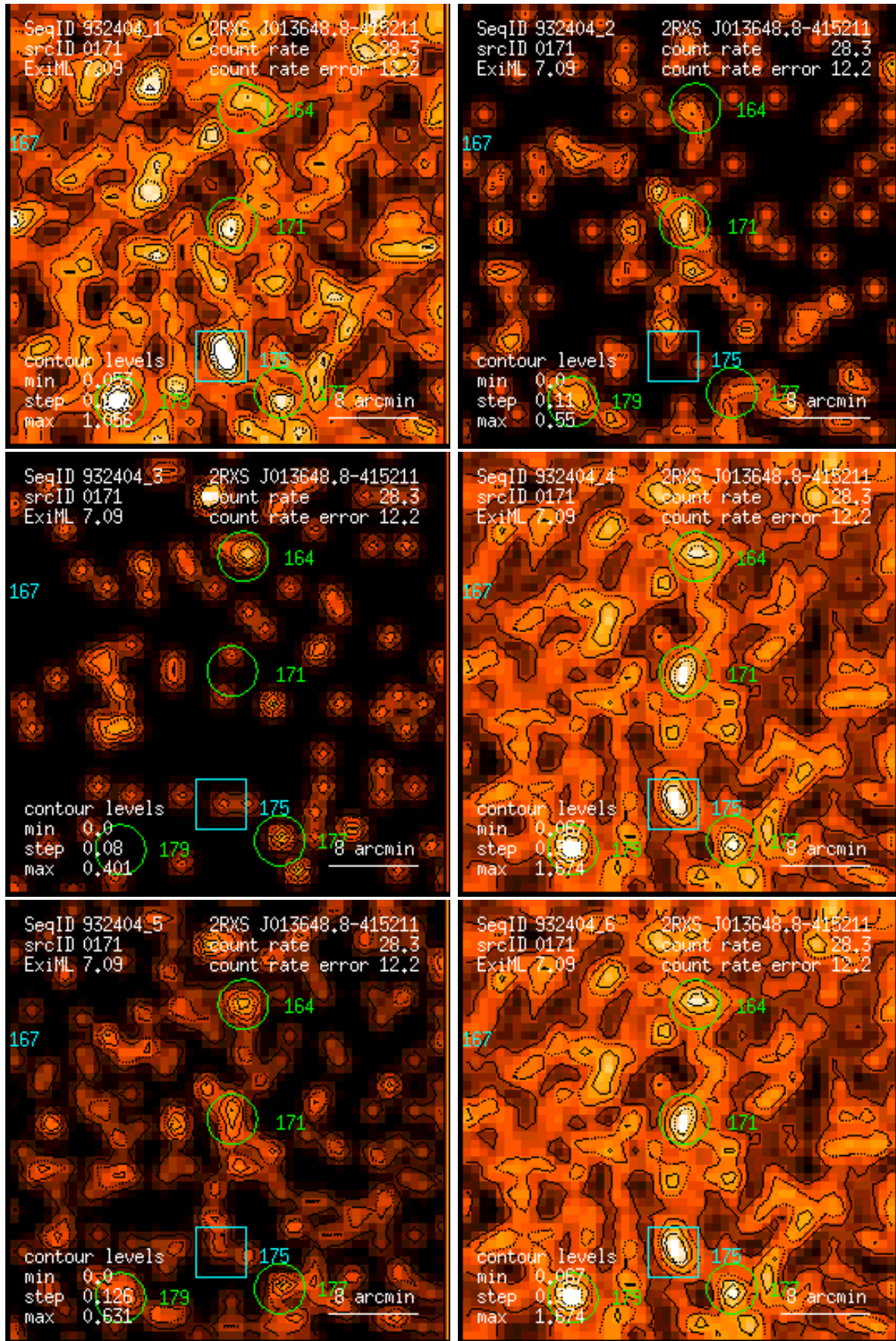
Figure 171: RASS 932404: detection 0171: band rate images, Gaussian filter: (1) PSPC channels 11 – 41, (2) 52 – 90, (3) 91 – 201, (4) 11 – 235, (5) 52 – 201, (6) 11 – 201. Broad band rates in counts/ks. Band rate contour levels in counts/ks/arcmin 2 .
