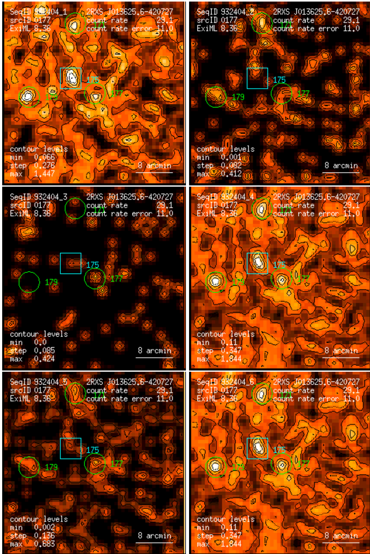
Figure 177: RASS 932404: detection 0177: band rate images, Gaussian filter: (1) PSPC channels 11 – 41, (2) 52 – 90, (3) 91 – 201, (4) 11 – 235, (5) 52 – 201, (6) 11 – 201. Broad band rates in counts/ks. Band rate contour levels in counts/ks/arcmin 2 .
